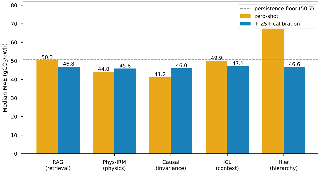
Five direction priors: complementary strengths (ZS+ equalizes them)
