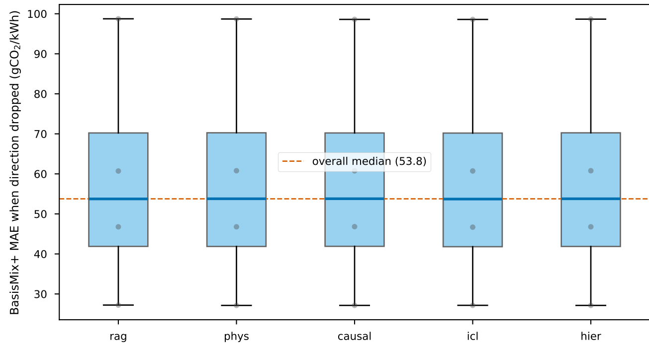
Drop-one ablation: removing any direction barely moves MAE (meta-learner is dead weight at zero-shot)
