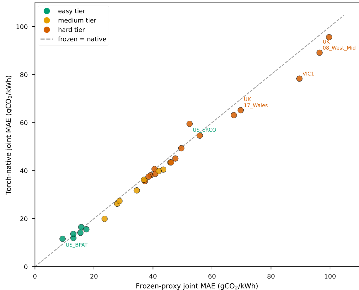
Per-region improvement: torch-native wins concentrate on hard grids
