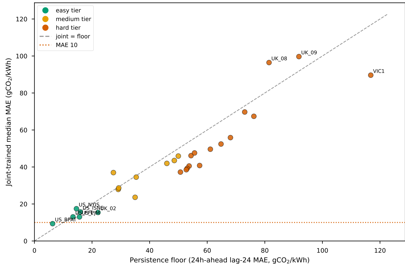
What bounds MAE: persistence floor drives error (Spearman \rho = 0.95 )
