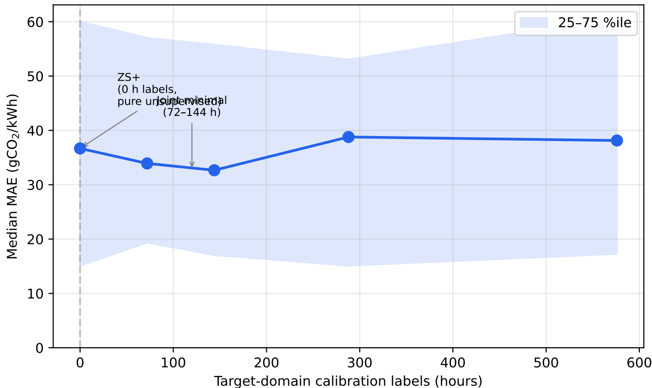
Calibration-data-amount curve: information-set stratification
