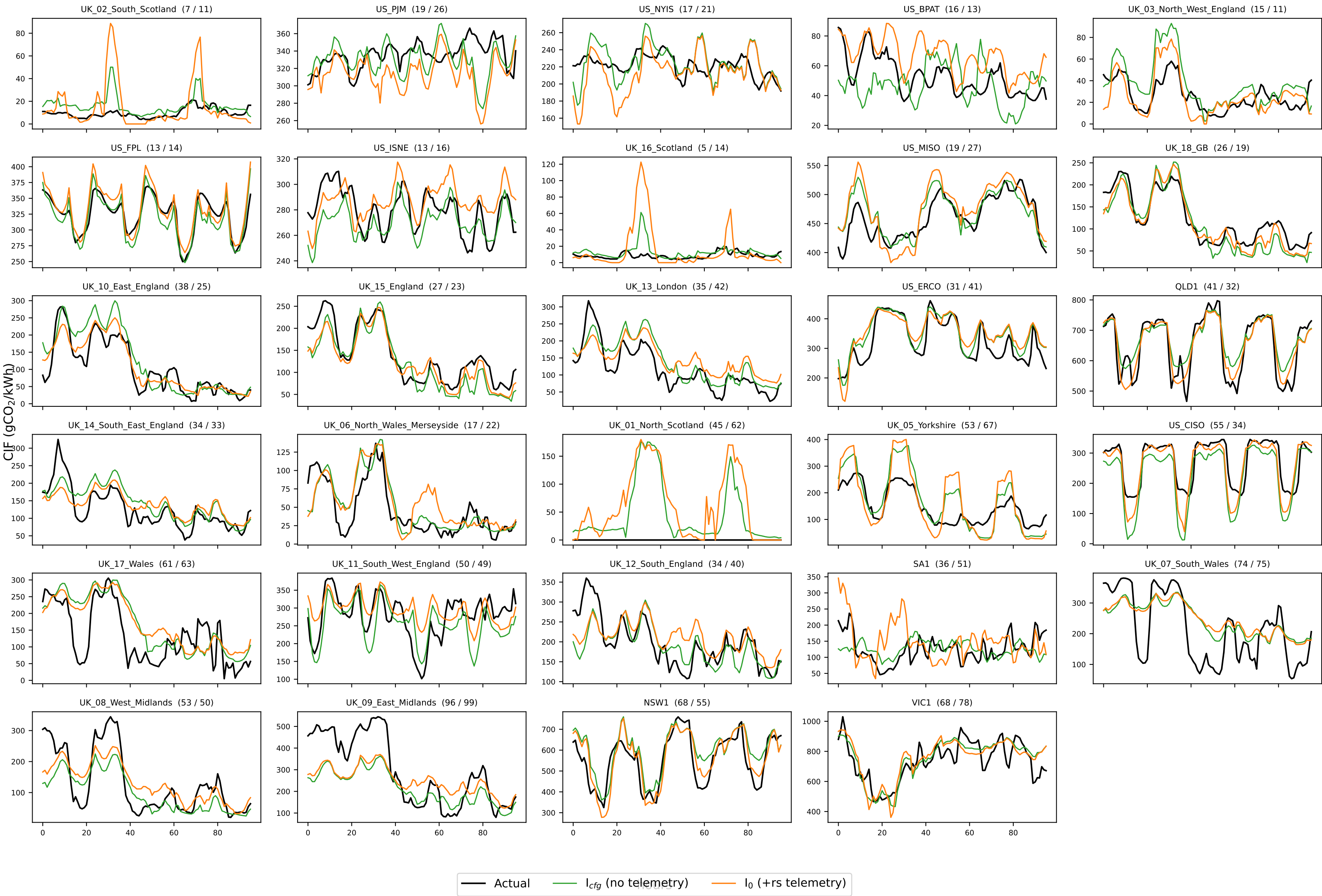
Day-ahead CIF, 29 regions — zero-telemetry (green) vs share telemetry (orange) panel title: l_{cfg} / l_0 MAE over the plotted 96 h; panels sorted by l_{cfg} ; FD-35 deployment v3
