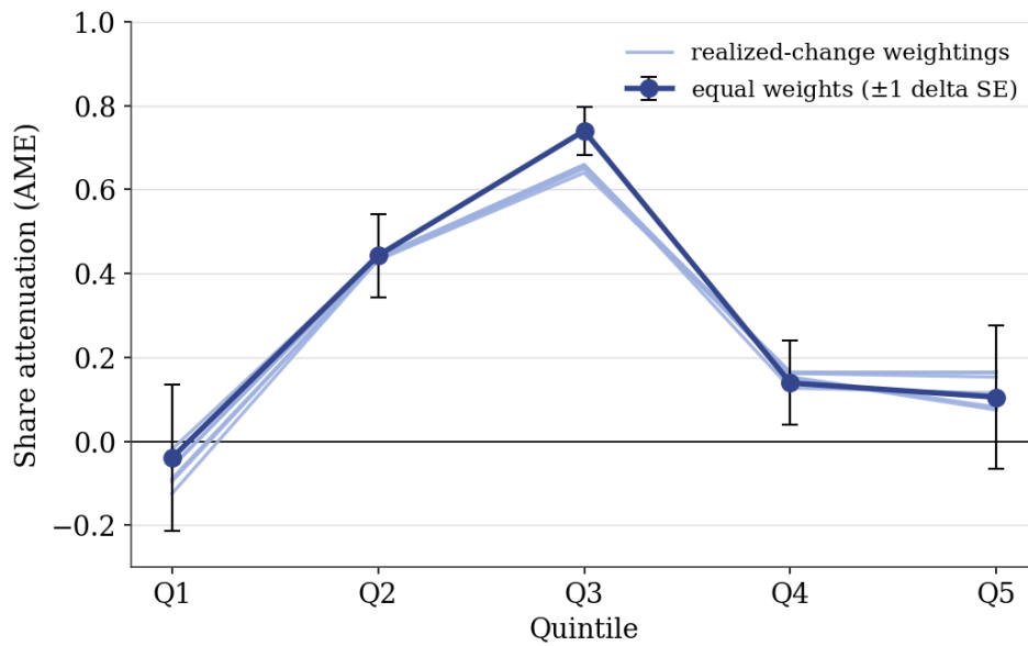
Figure 5: The Attenuation Structure, National Picture
