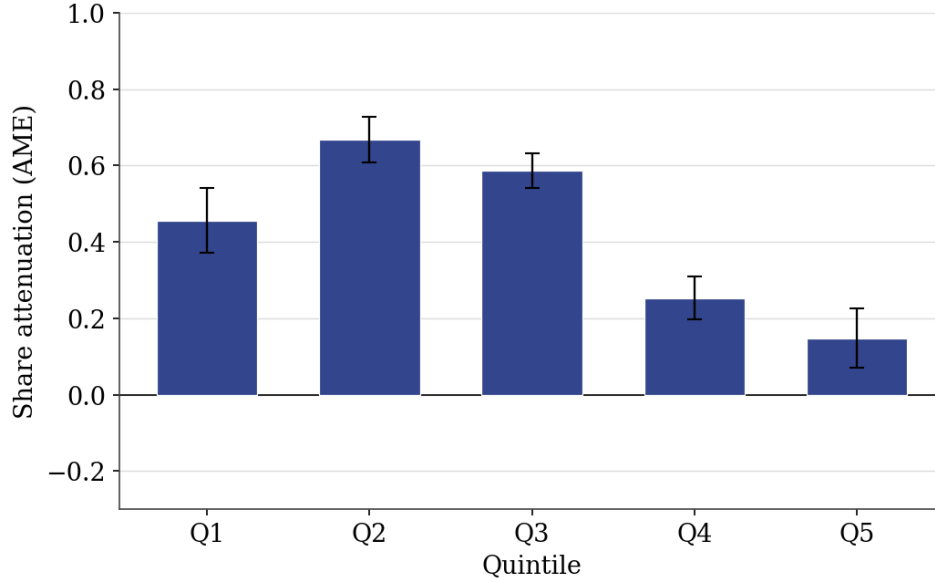
Figure 3: The Attenuation Structure (SUR Estimation)
