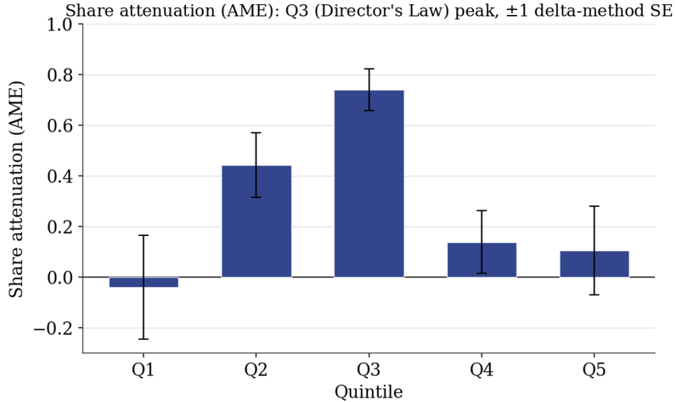
Figure 4: The Attenuation Structure (GMM Estimation)
