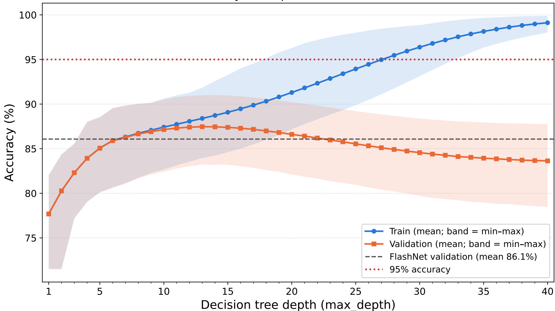
Decision tree accuracy vs. depth (trained on labels, 12 datasets)
