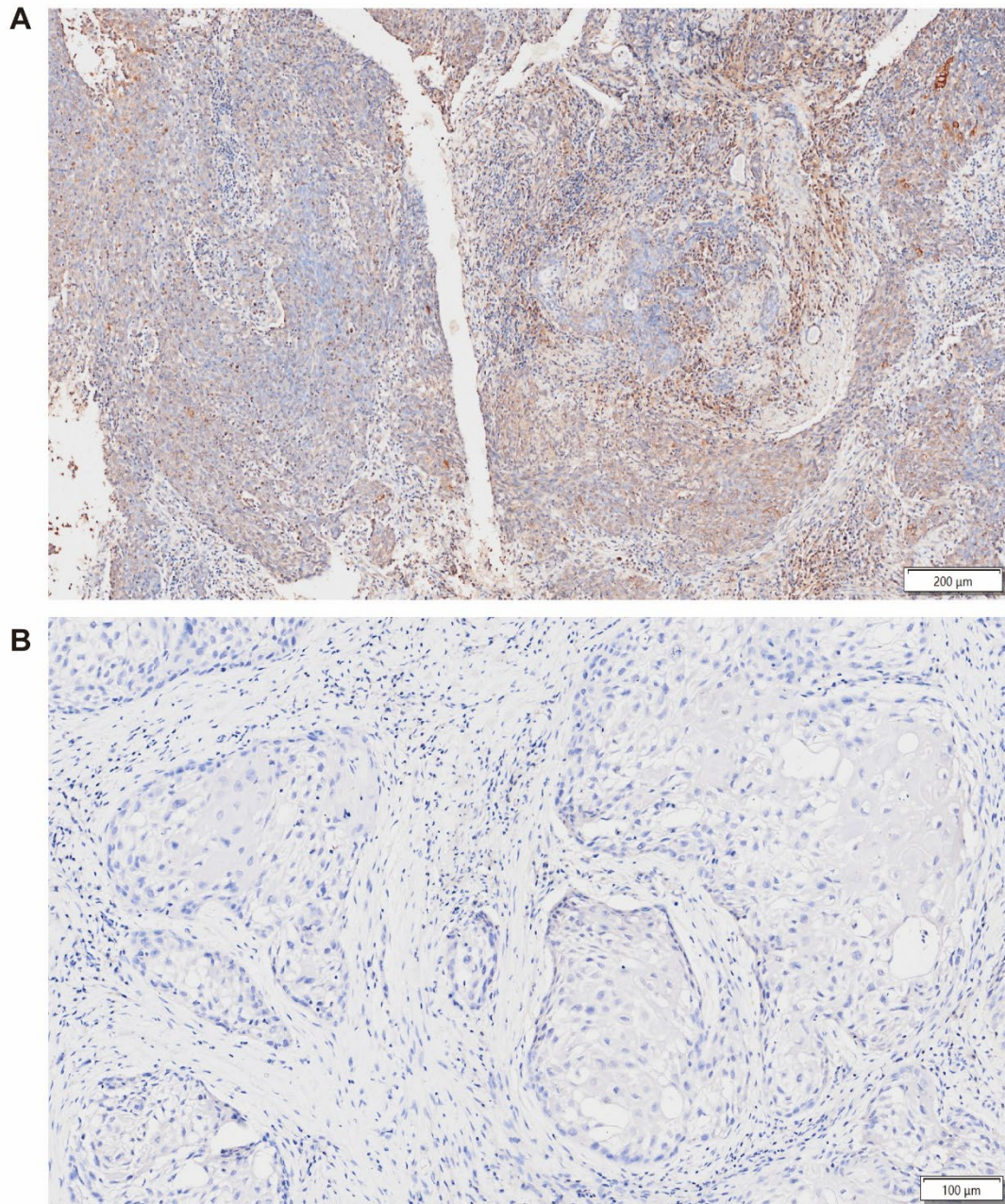
Supplementary Fig. S5. Positive and negative controls for CXCL10 immunostaining. (A) Positive control using human nasopharyngeal carcinoma tissue. (B) Negative control processed without the primary antibody.
