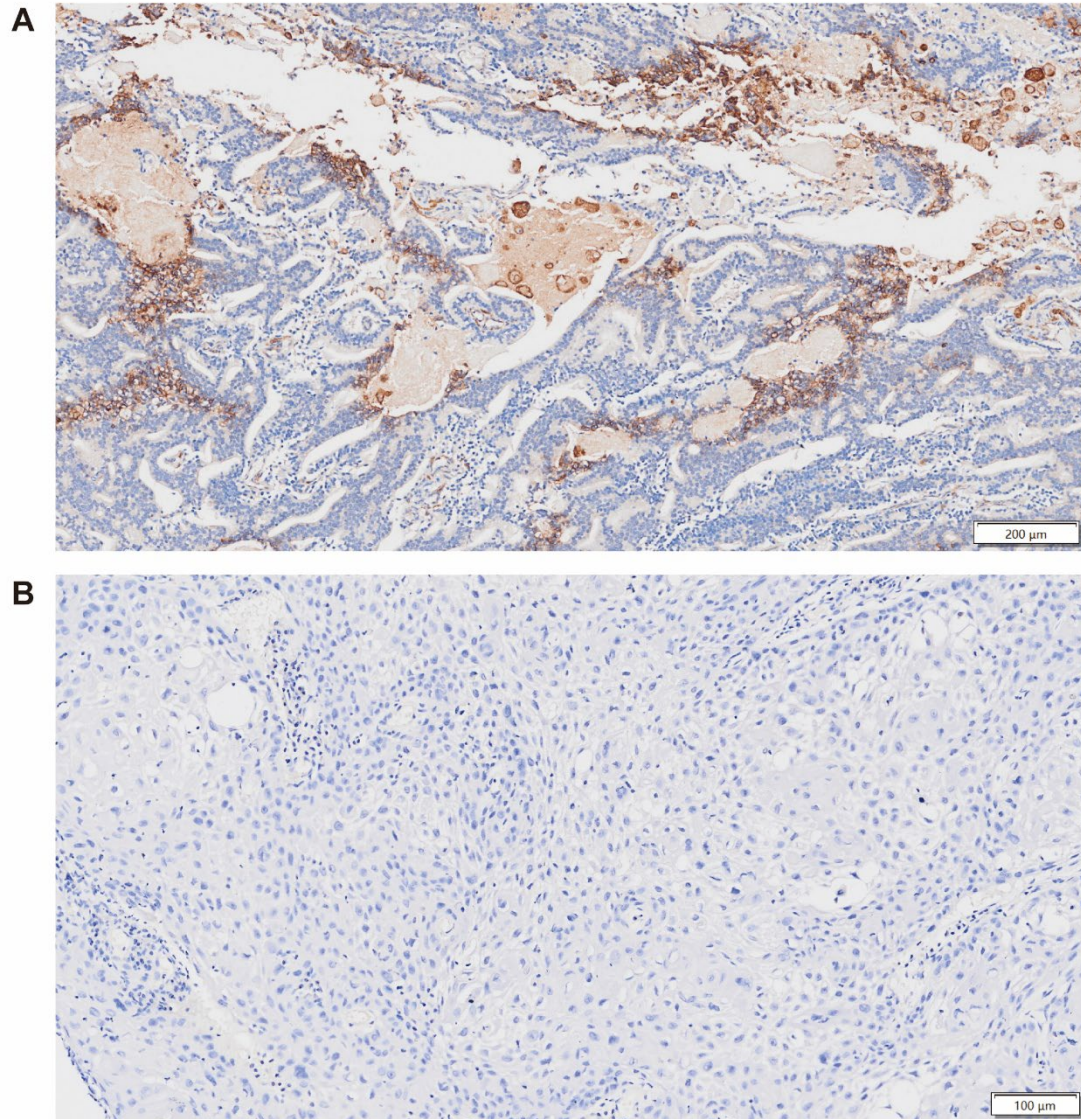
Supplementary Fig. S2. Positive and negative controls for monocarboxylate transporter 4 (MCT4) immunohistochemistry. (A) Positive control using human prostate tissue. (B) Negative control without the primary antibody.
