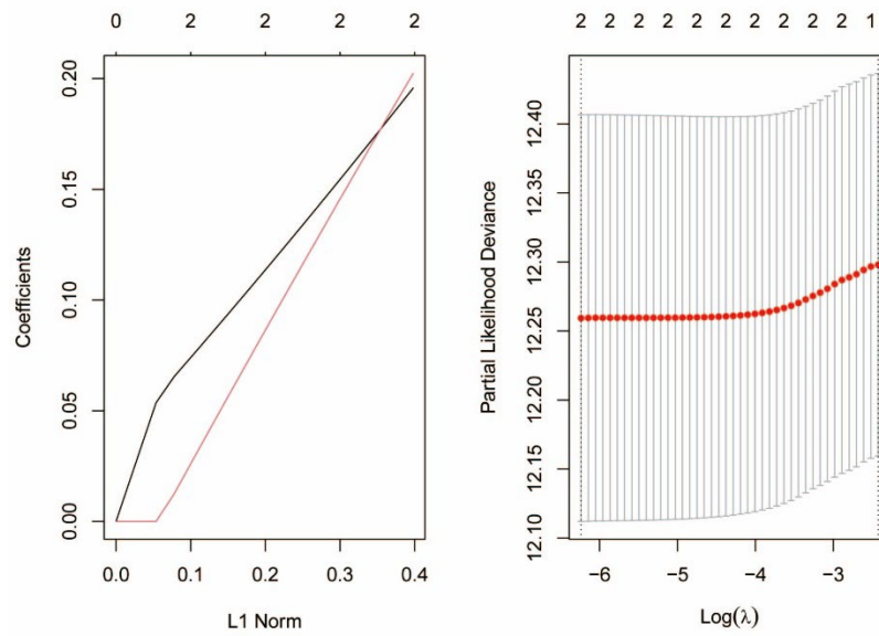
Supplementary Fig. S1. The LRS formula was constructed using a Lasso regression.
