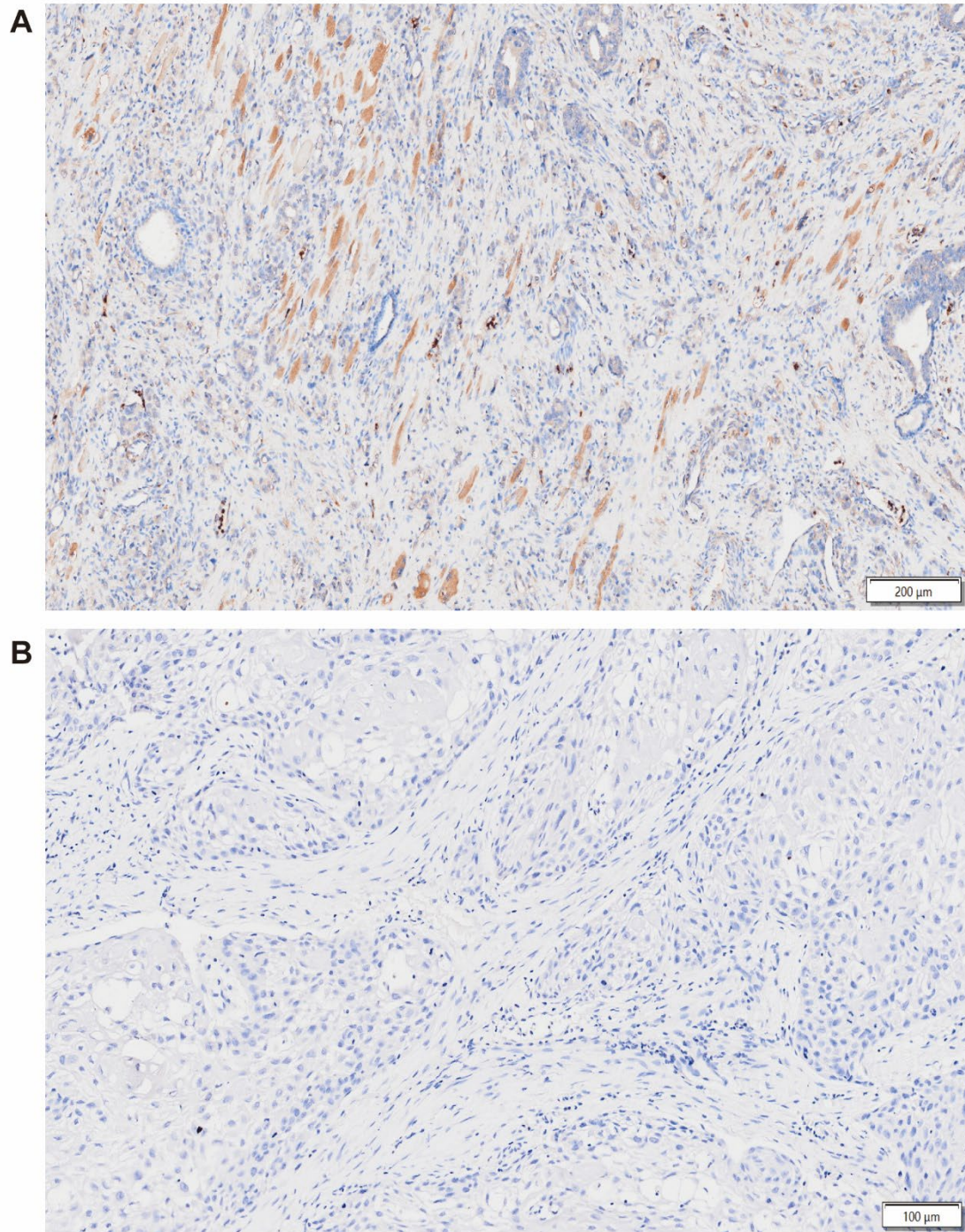
Supplementary Fig. S4. Positive and negative controls for CXCL9 immunostaining. (A) Positive control using human prostate cancer tissue. (B) Negative control processed without the primary antibody.
