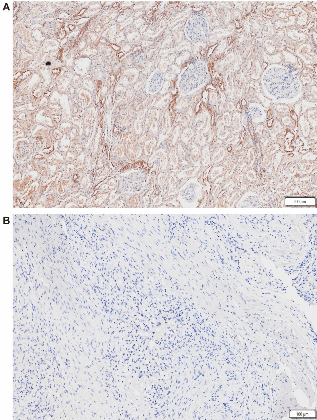
Supplementary Fig. S3. Positive and negative controls for glycogen phosphorylase L (PYGL) immunohistochemistry. (A) Positive control using human kidney tissue. (B) Negative control without the primary antibody.
