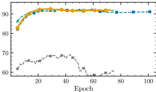
Recall (%)
