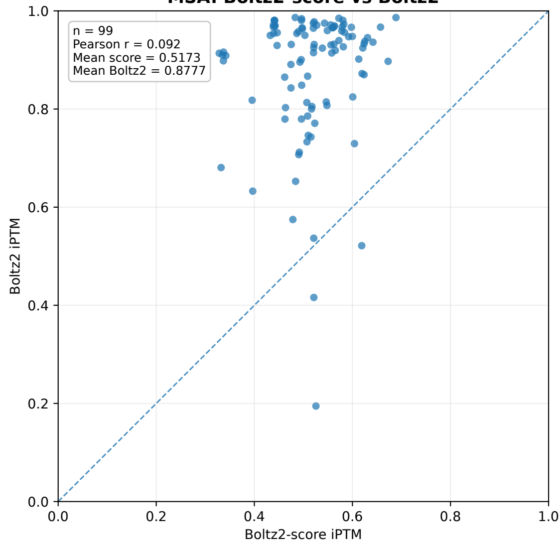
MSA: Boltz2-score vs Boltz2
