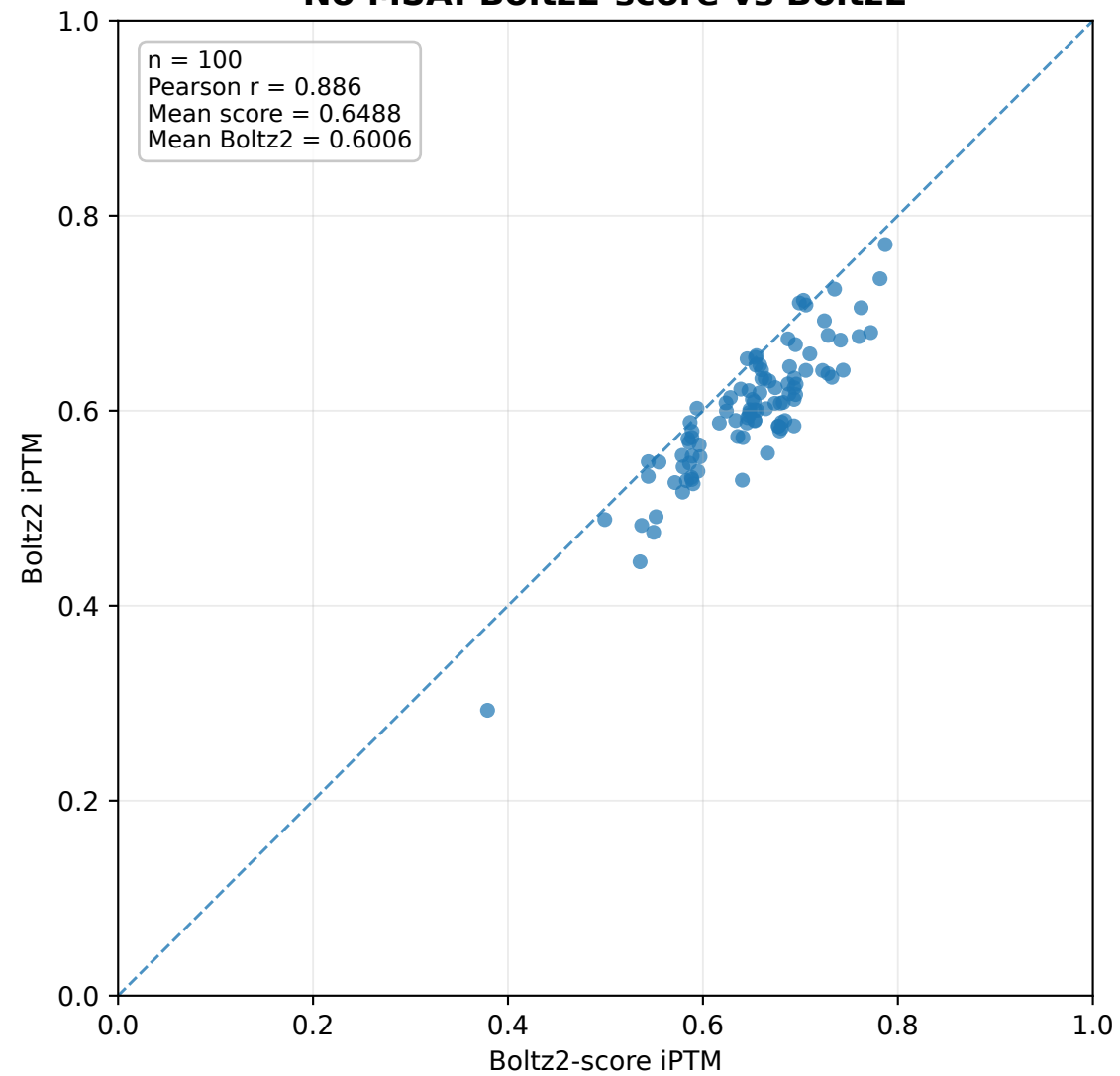
No MSA: Boltz2-score vs Boltz2
