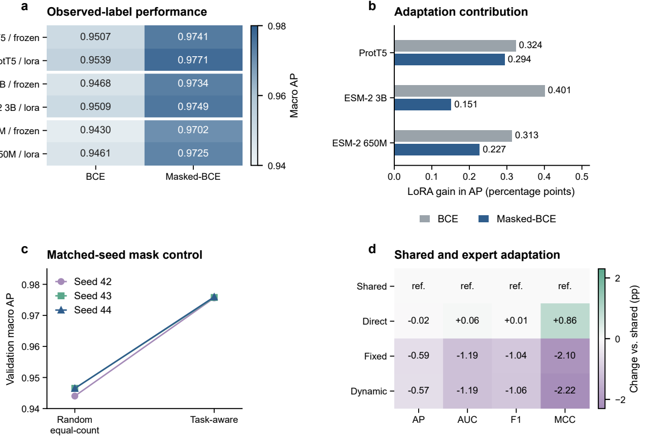
Fig. 2. Prediction ablations on observed validation labels. (a) Macro AP across backbones, adaptations, and losses. (b) LoRA gains over frozen encoders, in percentage points. (c) Matched seeds 42–44 in the separate mask-control experiment. (d) Expert-minus-shared metric differences, in percentage points; the shared row is the reference. Panels a, b, and d report single-run comparisons.
