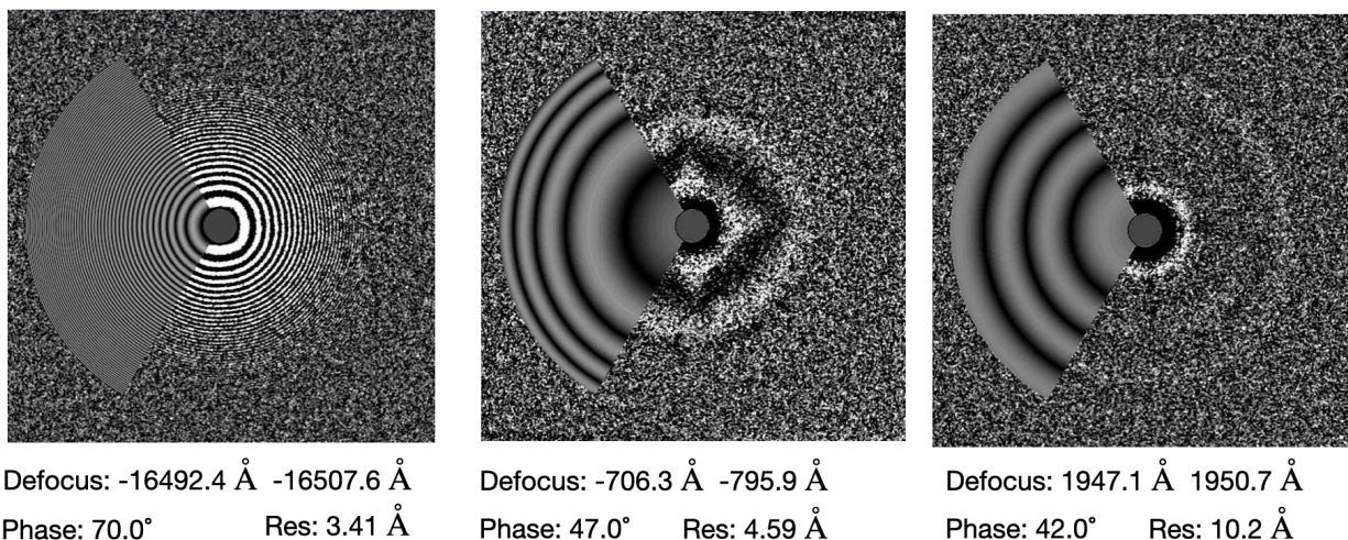
Fig. 2 Diagnostic images showing that GCtfFind delivered reliable CTF estimation from micrographs collected with overfocus and low defocus settings and different extra phase shifts.
