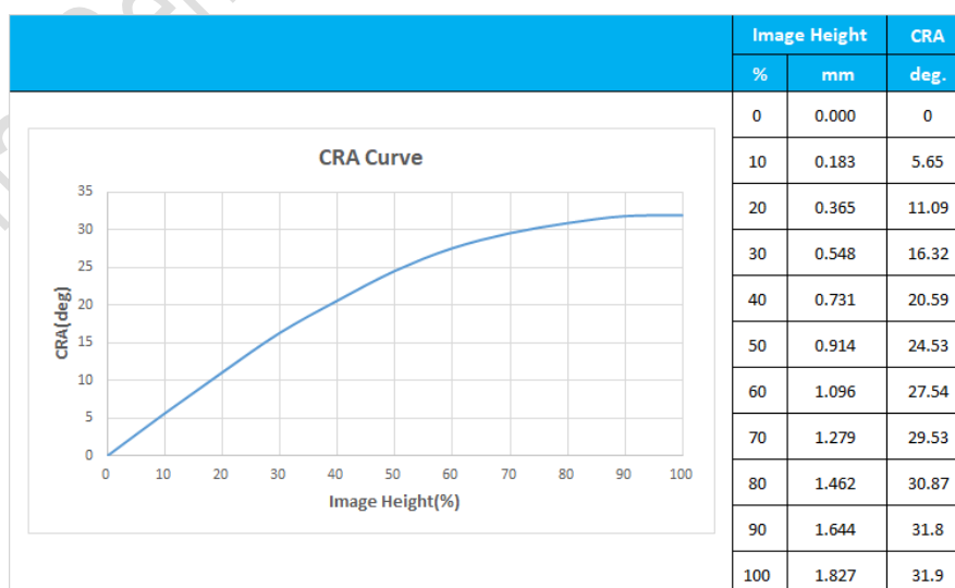
图 4-2 CRA Curve
