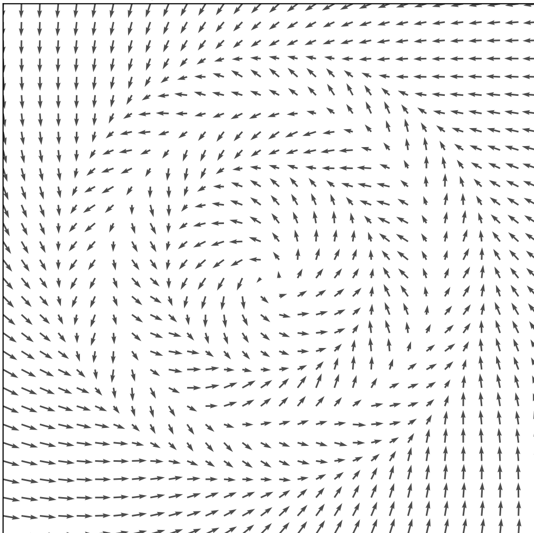
Trained Tangent Vector Field for doublecircles
