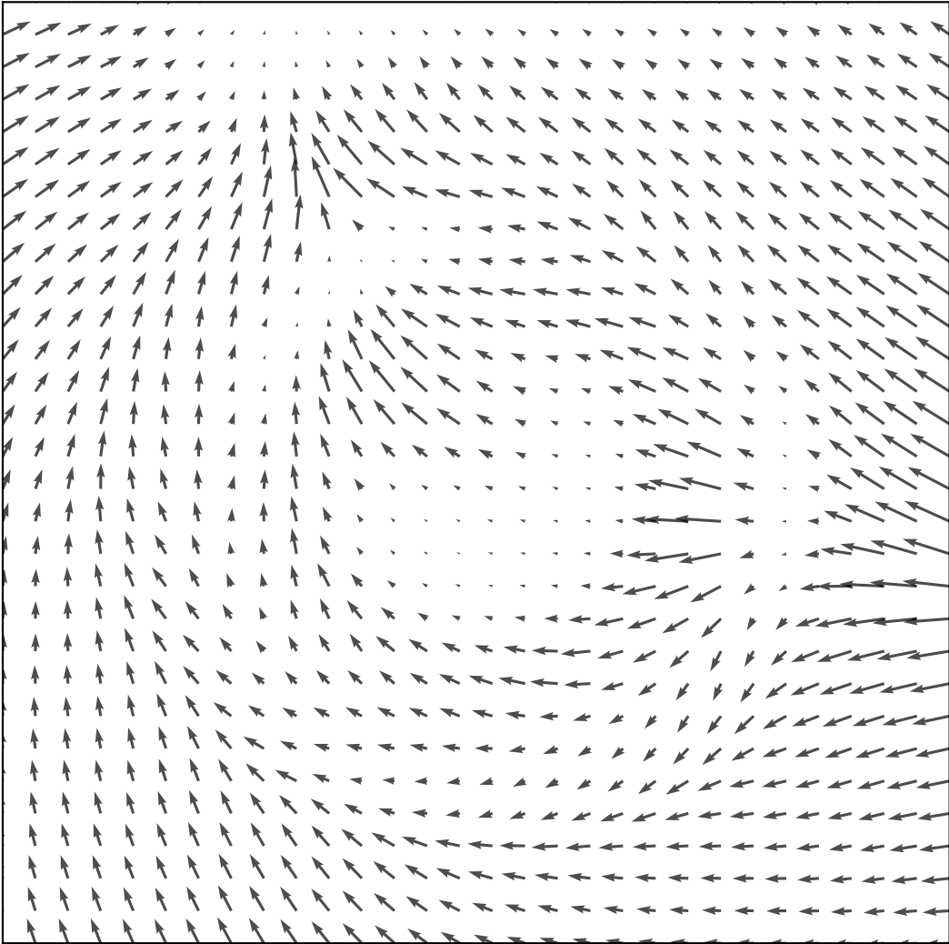
Trained Tangent Vector Field Without Orthogonality Constraint
