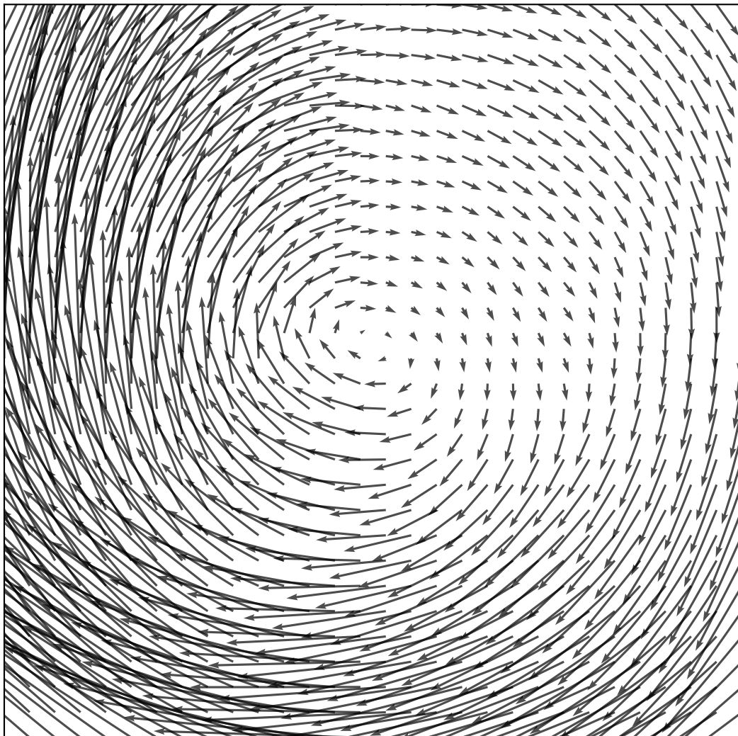
Trained Tangent Vector Field Without Unit-Norm Constraint
