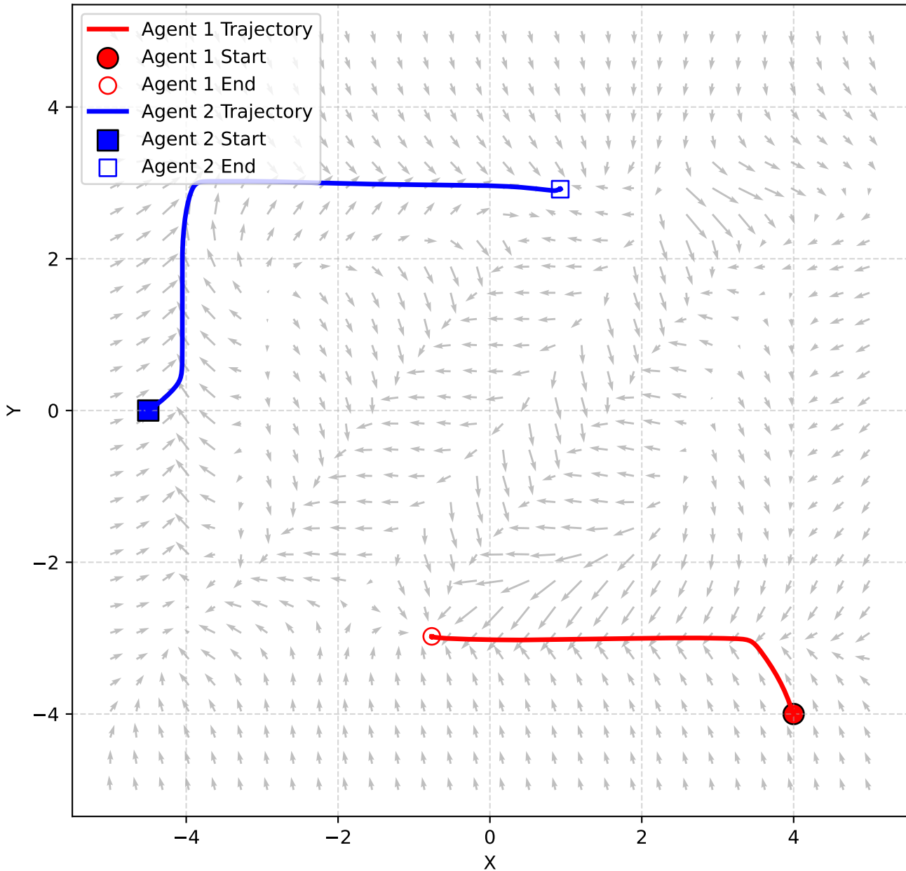
Robot Trajectories under Combined Field
