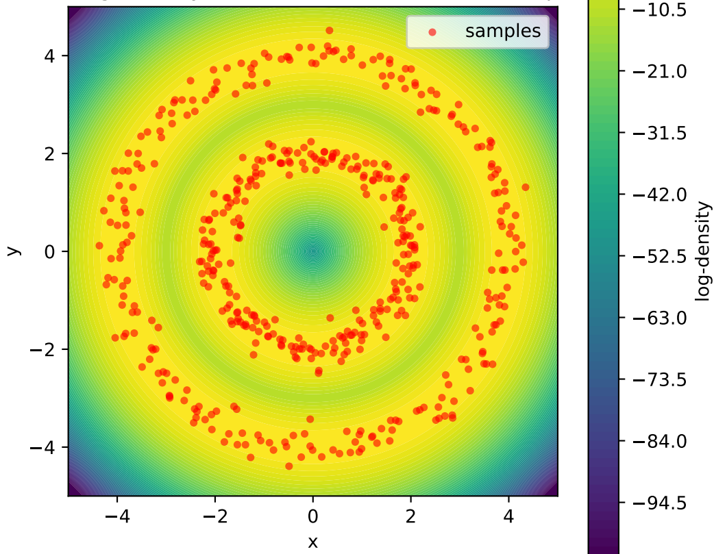
2D Log-Density of Concentric Circles with Samples
