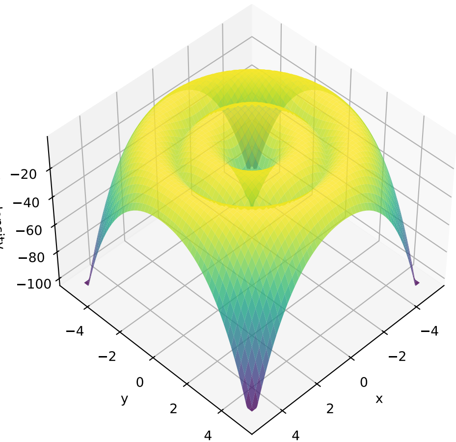
3D Log-Density of Concentric Circles with Samples
