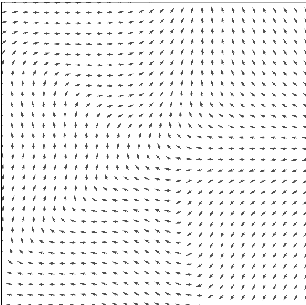
Trained Tangent Vector Field for Star5
