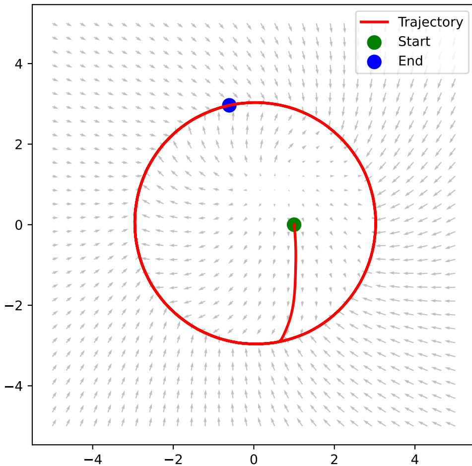
Robot Trajectory under Combined Field
