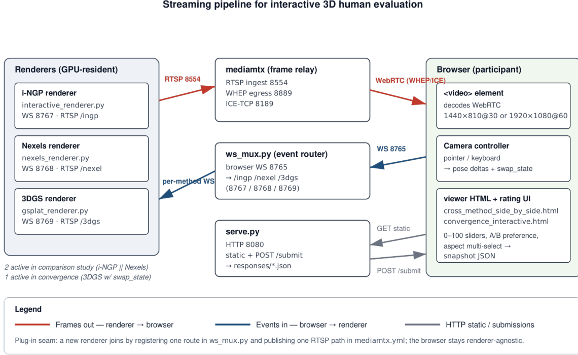
Figure 2: Streaming pipeline. The three renderers conform to a common contract (RTSP push for frames out, per-method WebSocket for events in); ws_mux.py and mediamtx between them keep the browser renderer-agnostic.
