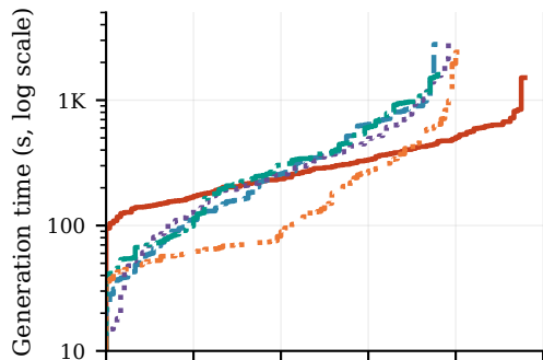
Generation completion
