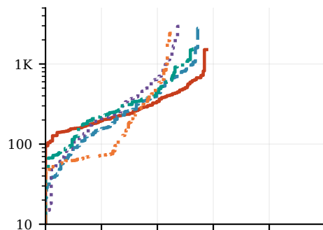
Behavioral score
