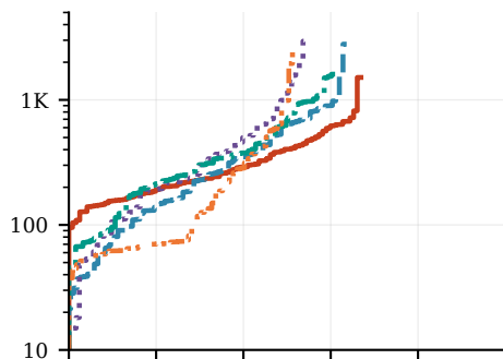
Operational score
