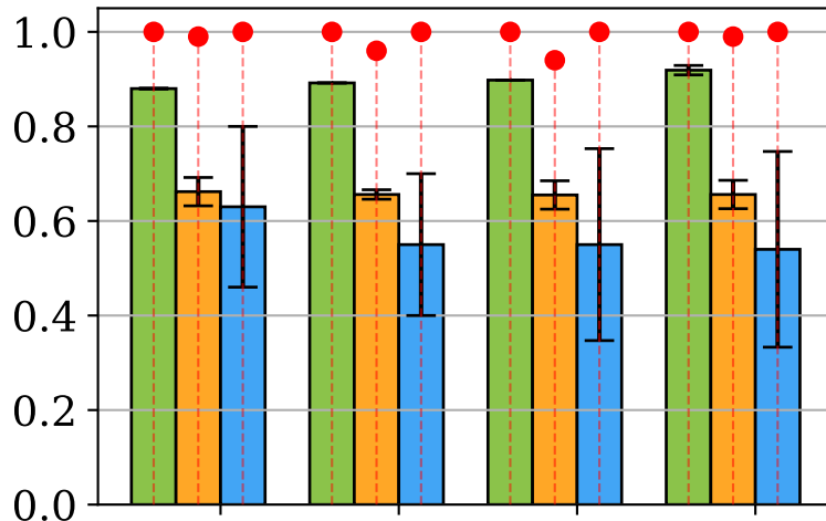
75% Node Reduction
