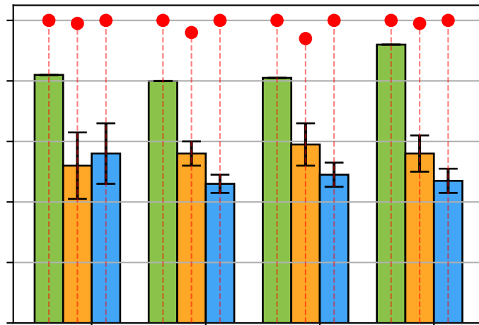
50% Node Reduction
