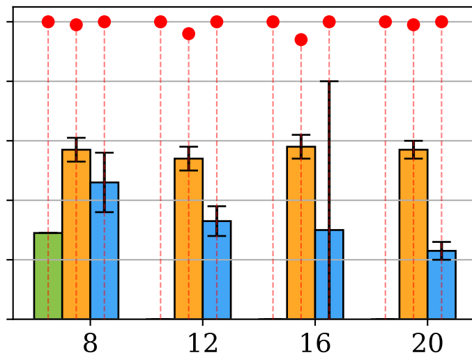
90% Node Reduction
