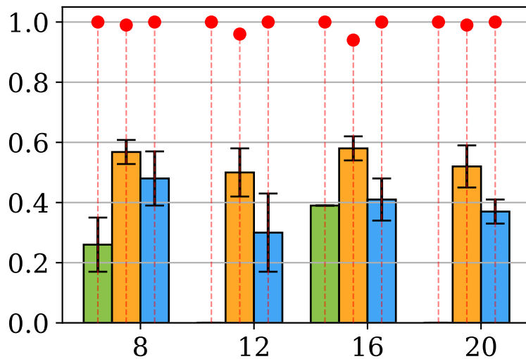
75% Node Reduction
