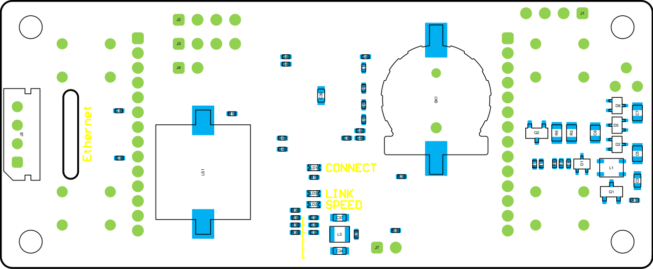
View from Bottom side (Scale 2:1)
