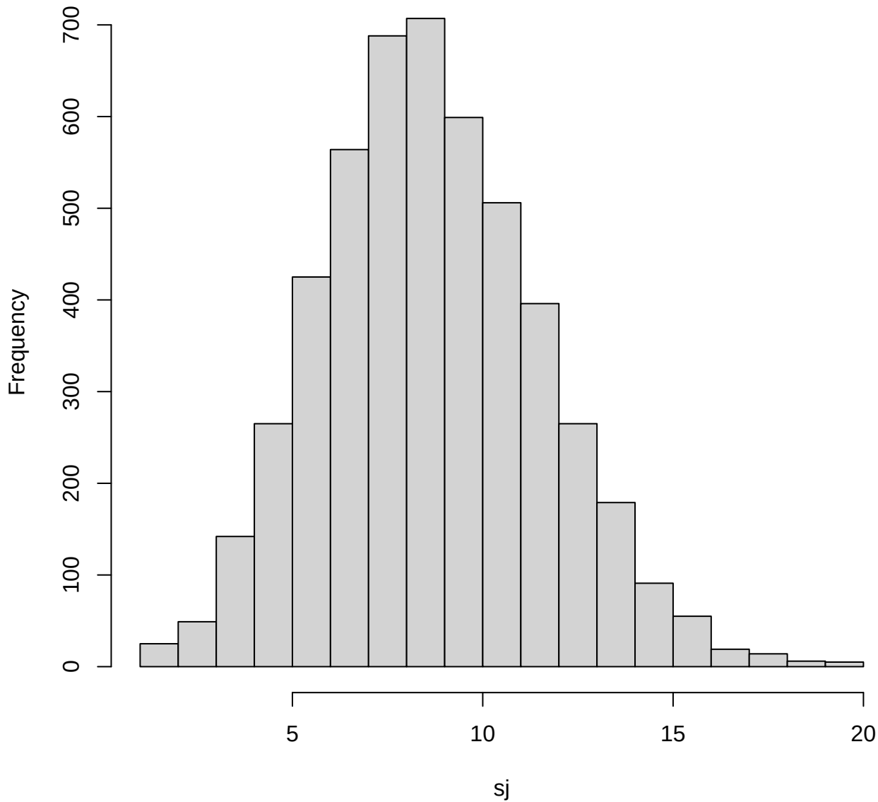
histogram of sj in state 4
