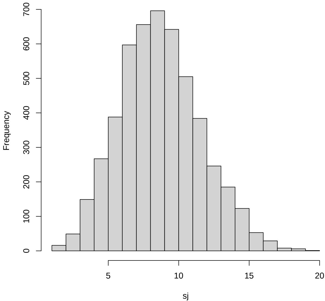
histogram of sj in state 1
