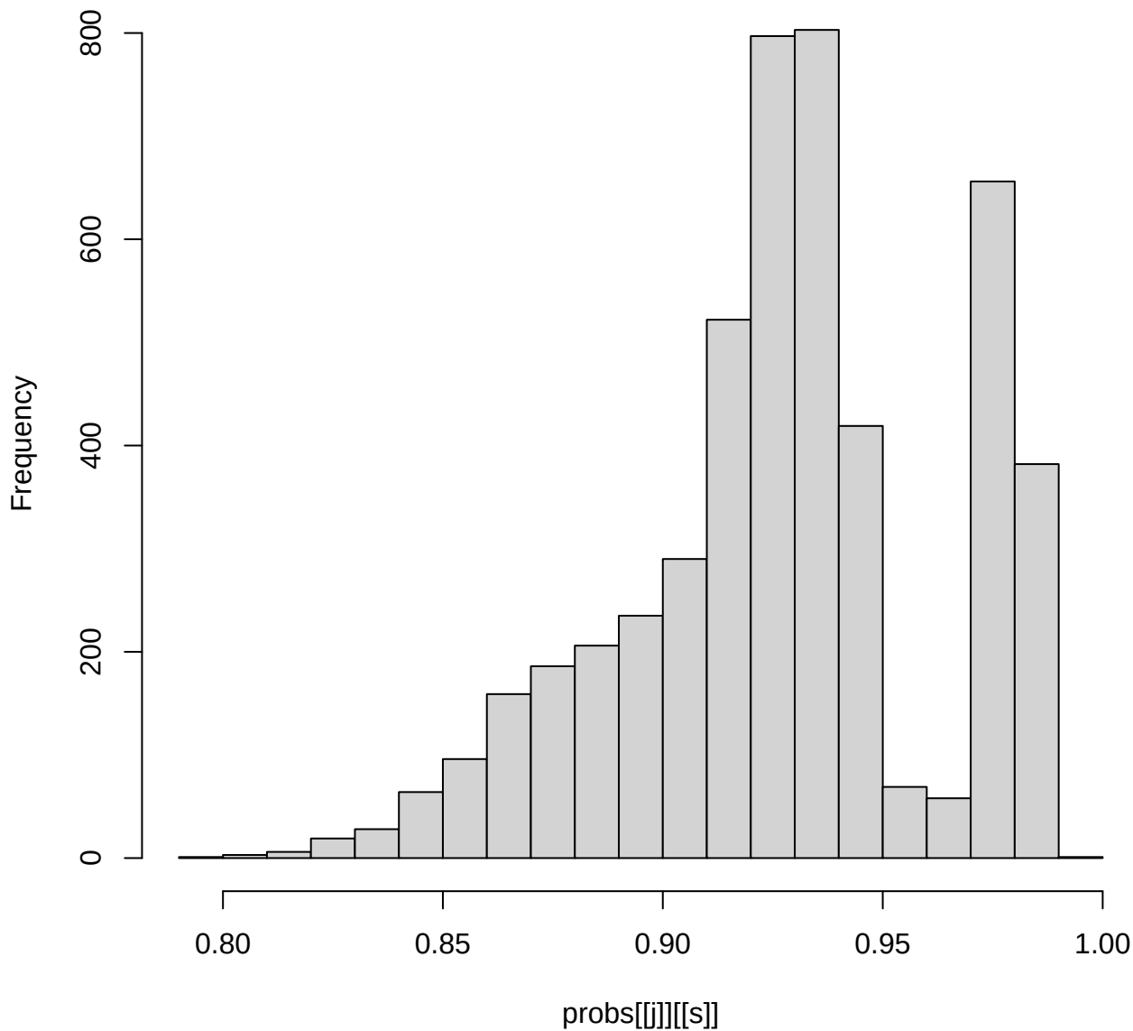
histogram of probs in state 1
