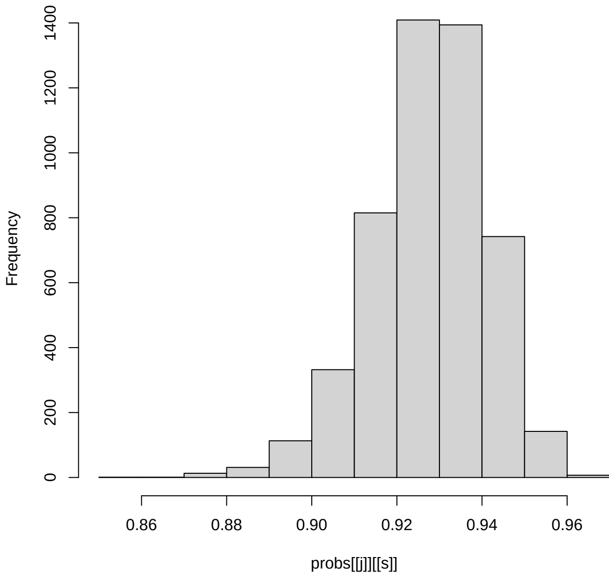
histogram of probs in state 4
