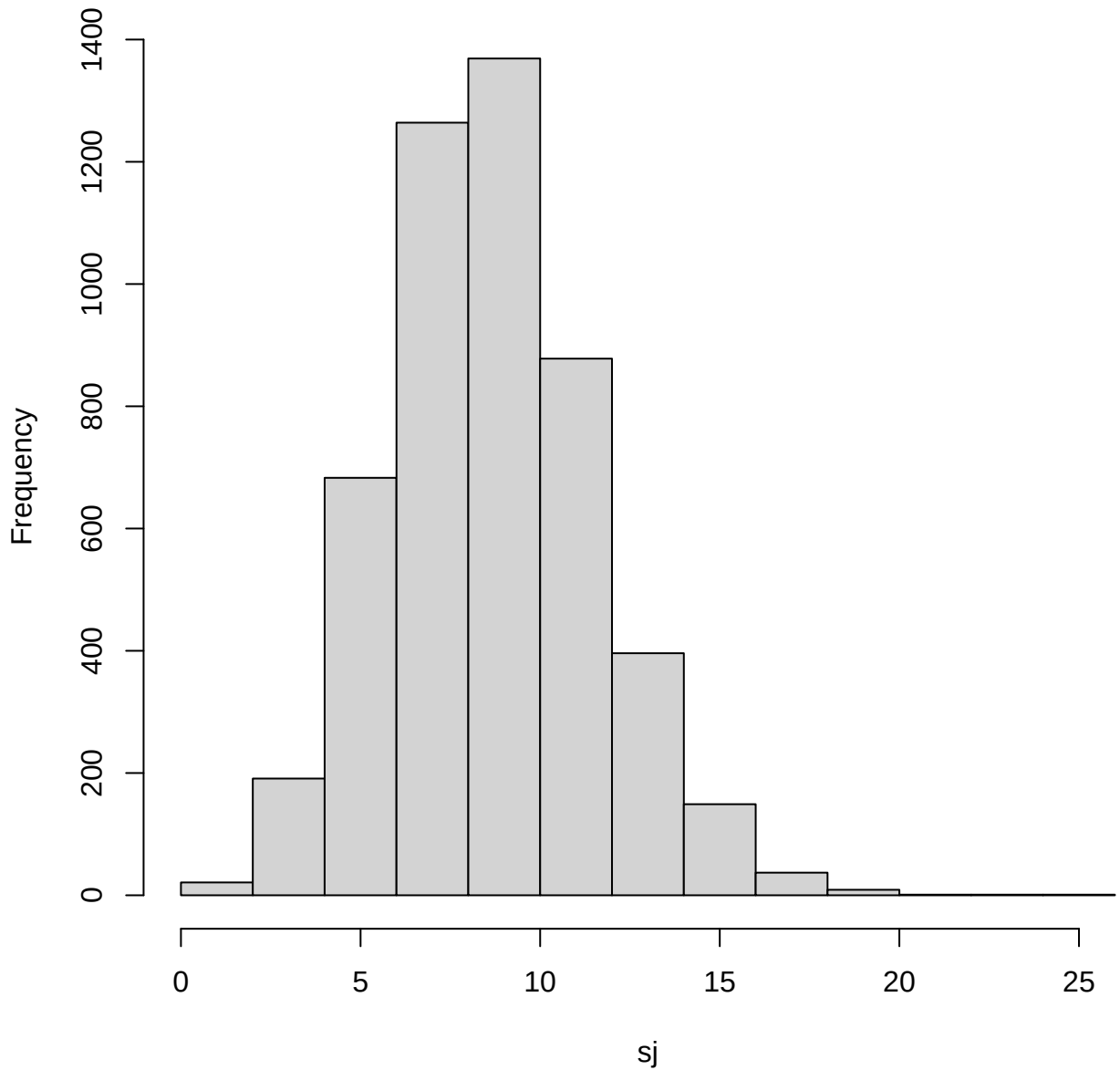
histogram of sj in state 2
