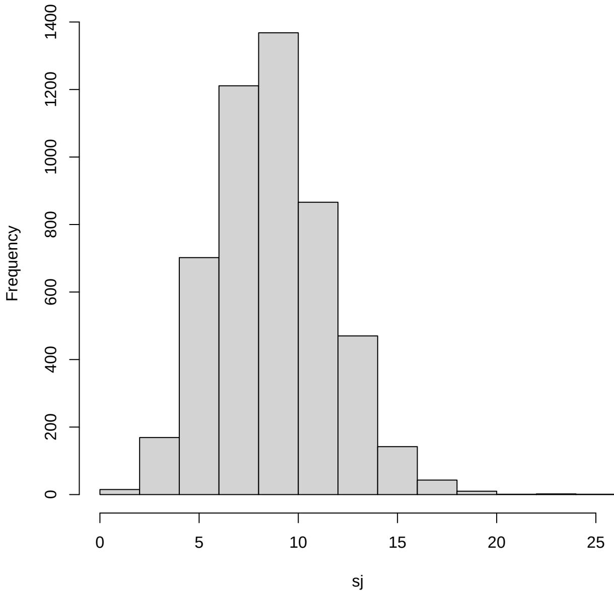
histogram of sj in state 1
