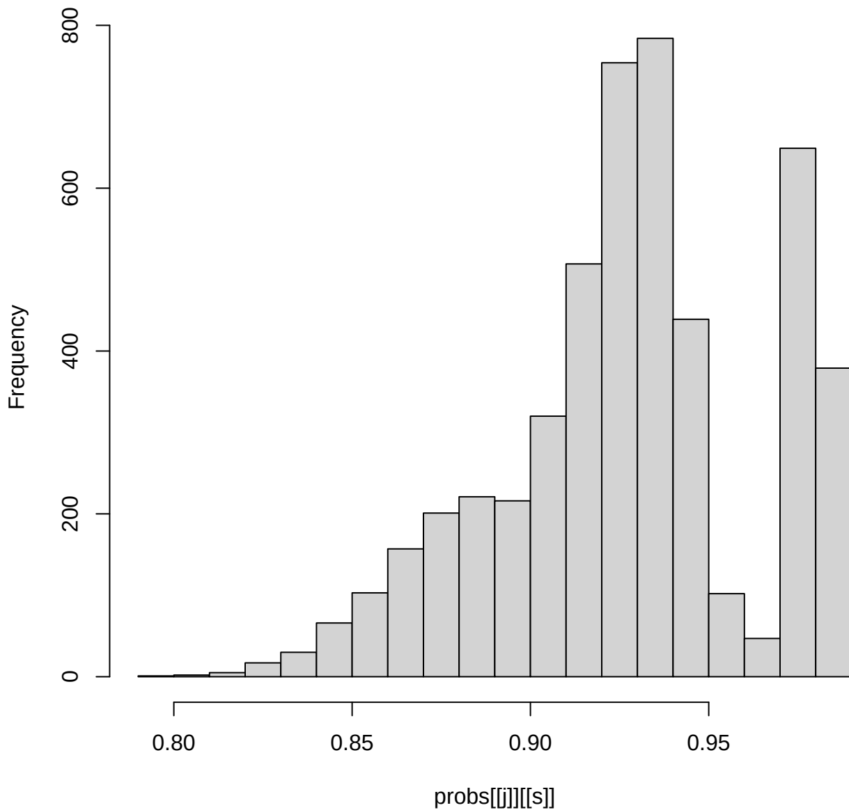
histogram of probs in state 3
