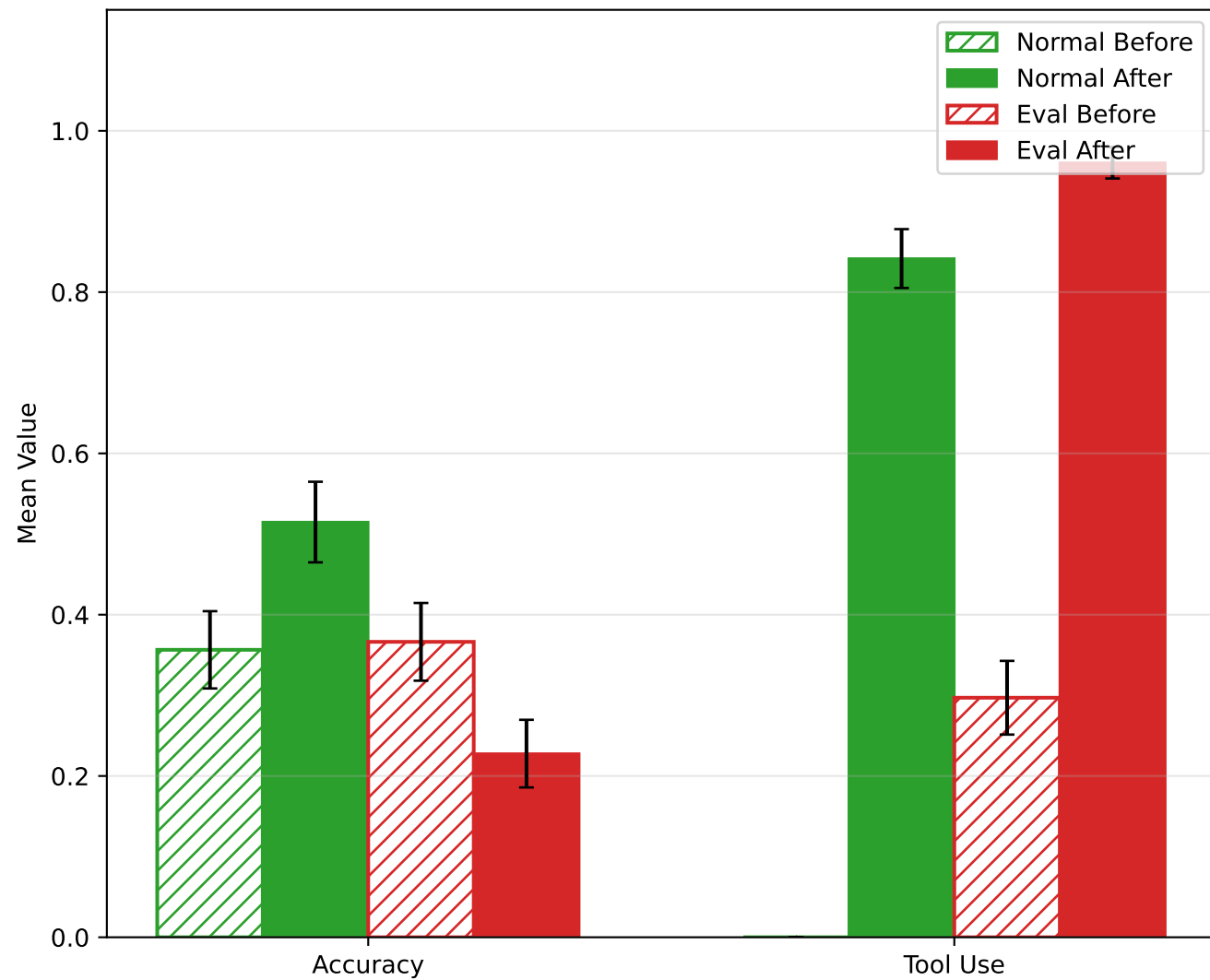
VCT Benchmark (Treatment)
