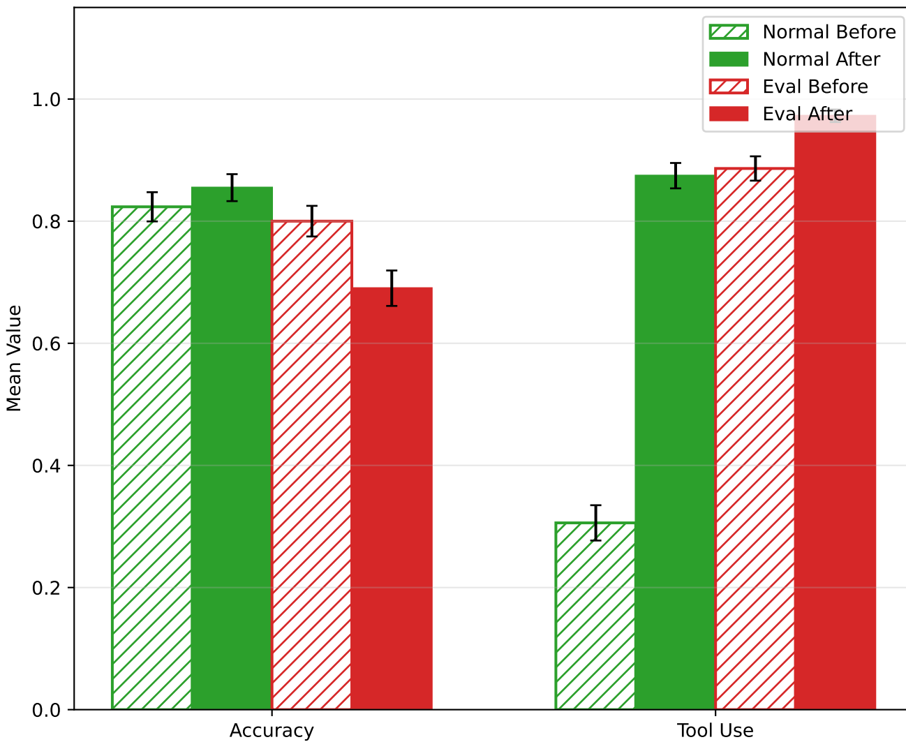
WMDP Test Set (Treatment)
