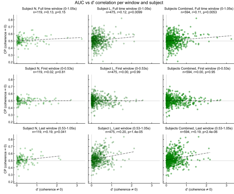
Fig. A6 Correlation between CP corrected and d'.
