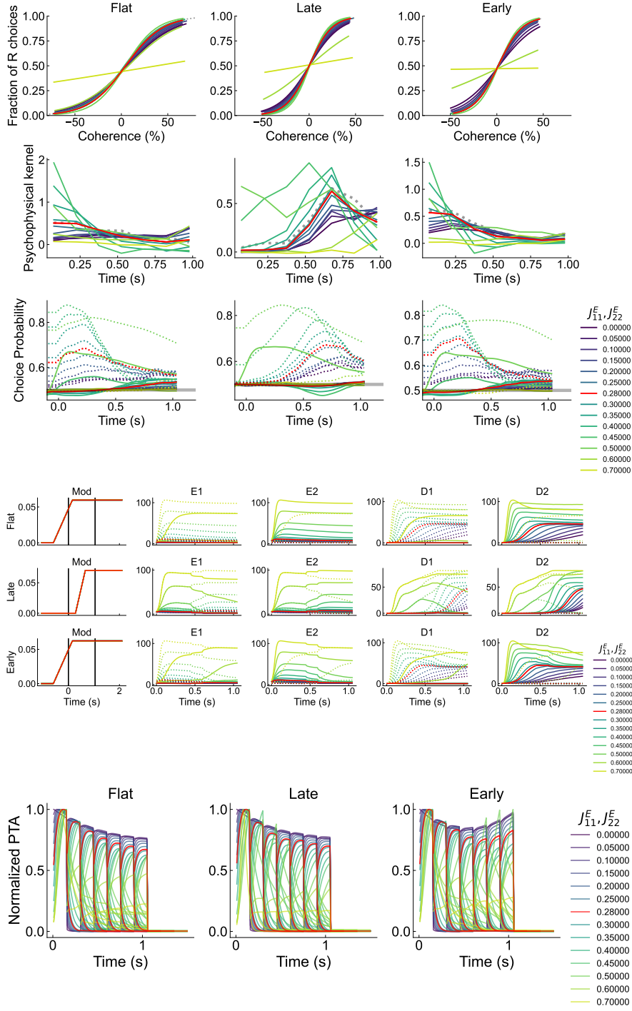
Fig. A15 Effects of varying J_{11}^E = J_{22}^E . Red indicates model output for optimized parameters. In CP plots, dotted lines indicate raw CP, solid lines indicate corrected CP. In firing rate plots, dotted lines indicate tuning to target 1, solid lines indicate tuning to target 2.
