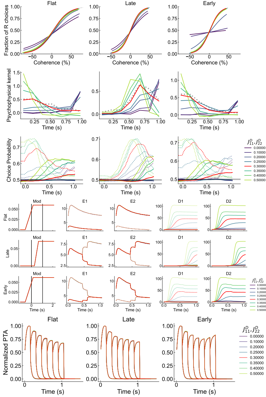
Fig. A17 Effects of varying J_{11}^D = J_{22}^D . Red indicates model output for optimized parameters. In CP plots, dotted lines indicate raw CP, solid lines indicate corrected CP. In firing rate plots, dotted lines indicate tuning to target 1, solid lines indicate tuning to target 2.
