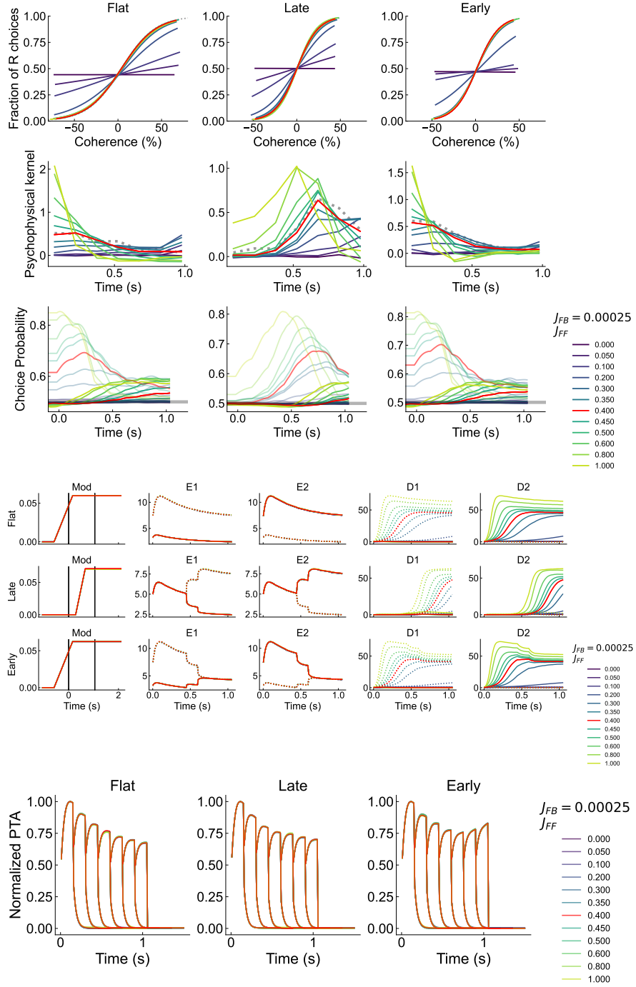
Fig. A10 Effects of varying J_{FF} . Red indicates model output for optimized parameters. In CP plots, dotted lines indicate raw CP, solid lines indicate corrected CP. In firing rate plots, dotted lines indicate tuning to target 1, solid lines indicate tuning to target 2.
