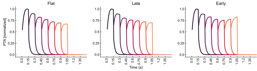
Fig. A8 PTA evoked by motion pulses in the neural network model. PTA averaged across sessions for each task condition, computed over the weighted sum of firing rate simulated.
