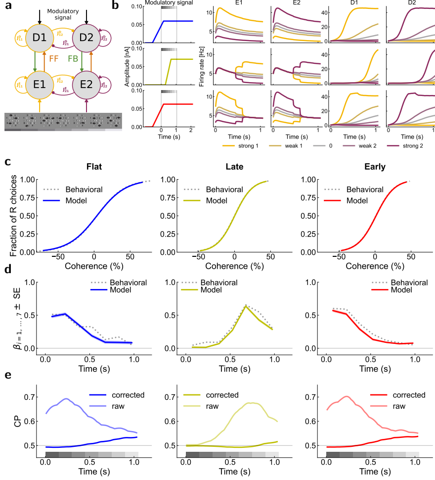
Fig. 3 Two-area neural network model and simulation results. a. Two-areas model architecture consisting of two pairs of stimulus-selective neural populations, respectively tuned to target 1 or target 2. Populations labelled with E indicate sensory encoding, D indicates decision encoding. Arrows indicate inputs and excitatory connections ( J_{11}^E, J_{22}^E, J_{11}^D, J_{22}^D ), circled edges indicate inhibitory connections ( J_{12}^E, J_{21}^E, J_{12}^D, J_{21}^D ). b. Modulatory signals and firing rates of the two pairs of populations in the three temporal weighting conditions generated with optimized parameters. From left to right: Modulatory signals, E1, E2 and D1, D2. Top to bottom: flat (blue), late (yellow), early (red). c. Logistic fits for choices generated by the two-paired populations model in the three temporal weighting conditions (solid) compared to behavioral performances combined between the two subjects (dotted). d. PKs based on simulated choices in the three temporal weighting conditions (solid) compared to behavioral PKs for data combined between the two subjects (dotted). e. CP raw (shaded lines) and corrected (solid lines) in sensory population firing rates for the three temporal weighting conditions in zero pulse-average coherence trials. b–e. Simulations included 10000 trials for each of the five coherence levels (strong 1, weak 1, 0, weak 2, strong 2).
