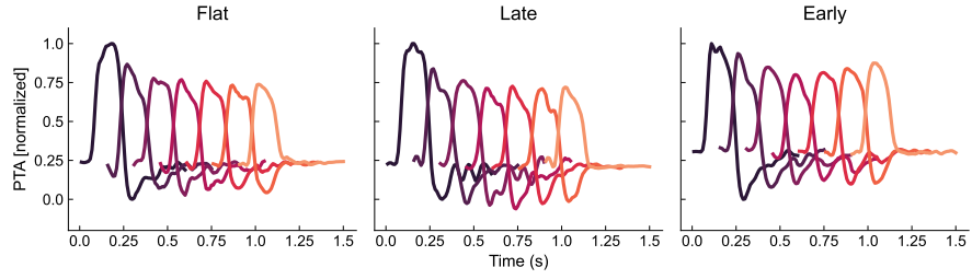
Fig. A7 PTA evoked by motion pulses in MT data. PTA averaged across sessions for each task condition, computed over the weighted sum of firing rates for cells recorded in each session.
