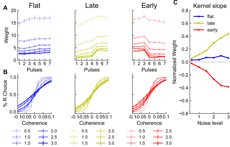
Fig. 4 Non-uniform temporal weighting emerges as an optimal strategy in task-trained RNNs. RNNs were trained independently on the flat, late and early conditions at noise levels \sigma_S = [0.5, 3] (light to dark colors). Curves show the mean across 10 networks per condition and noise level. a. Psychophysical kernels (logistic regression weights of the seven pulses). b. Psychometric functions (fraction of right choices vs. motion strength). c. PK slope as a function of noise level (positive values indicate recency, negative values primacy and zero uniform weighting).
