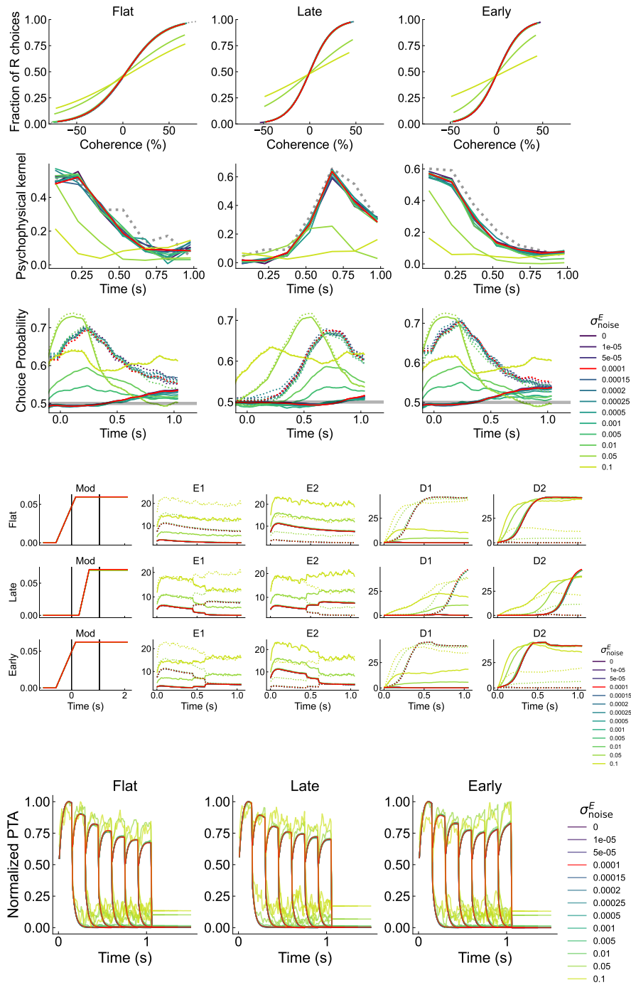
Fig. A19 Effects of varying \sigma_{\text{noise}}^E . Red indicates model output for optimized parameters. In CP plots, dotted lines indicate raw CP, solid lines indicate corrected CP. In firing rate plots, dotted lines indicate tuning to target 1, solid lines indicate tuning to target 2.
