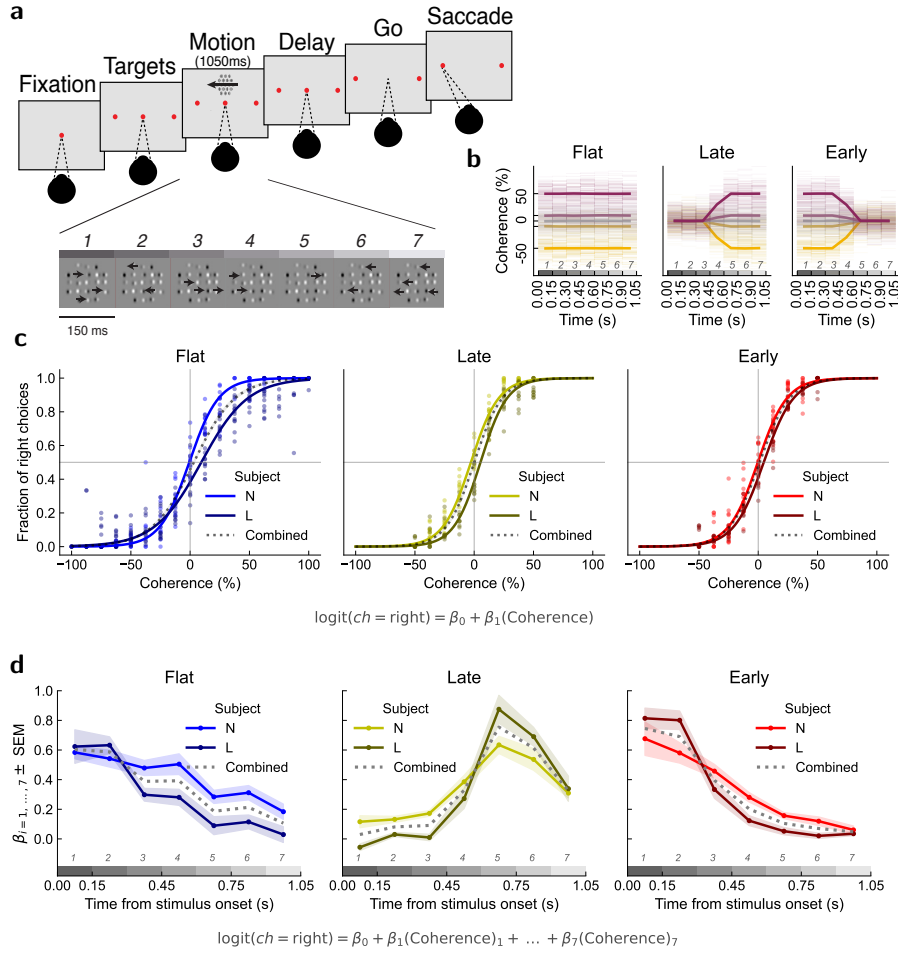
Fig. 1 Behavioral paradigm and psychophysical characterization of temporal weighting conditions. a. Perceptual motion-discrimination task. Trials start with a fixation point at the center of the screen. Once fixation is acquired, two choice targets appeared on opposite sides. The visual stimuli consist of a sequence of seven consecutive motion pulses, each lasting 150 ms, with independently changing direction and coherence. The signed coherence is given by the proportion of drifting Gabor elements, with positive coherence indicating rightward motion. Following stimulus presentation and a delay period subjects report their choice about the net motion direction with a saccadic eye movement to a choice target. b. Example stimulus time courses showing randomly generated motion strength and coherence across time for the three task conditions (“Flat”, “Late”, “Early”). c. Psychometric functions showing the fraction of choices toward right target (positive coherence) versus net motion direction coherence. Dots correspond to average fractions in individual sessions. Solid lines are logistic fits, pooled across sessions for each of the two subjects. d. Psychophysical kernels (PK; mean \pm SEM across sessions), quantified by the logistic regression weight [\beta_1, \dots, \beta_7] of each pulse. c–d. Gray dotted lines indicate results from fits obtained by pooling trials across sessions and subjects.
