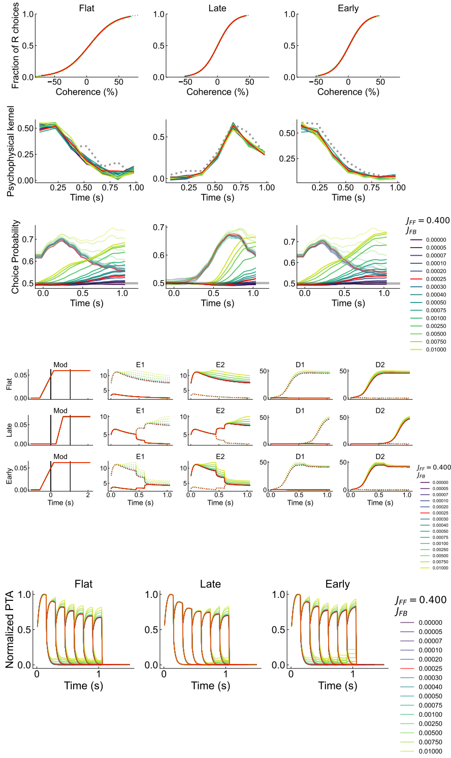
Fig. A11 Effects of varying J_{FB} . Red indicates model output for optimized parameters. In CP plots, dotted lines indicate raw CP, solid lines indicate corrected CP. In firing rate plots, dotted lines indicate tuning to target 1, solid lines indicate tuning to target 2.
