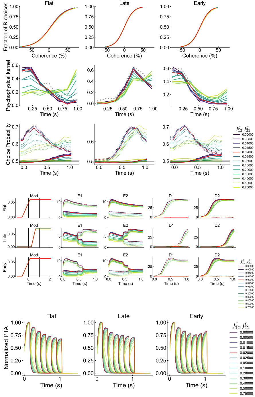
Fig. A16 Effects of varying J_{12}^E = J_{21}^E . Red indicates model output for optimized parameters. In CP plots, dotted lines indicate raw CP, solid lines indicate corrected CP. In firing rate plots, dotted lines indicate tuning to target 1, solid lines indicate tuning to target 2.
