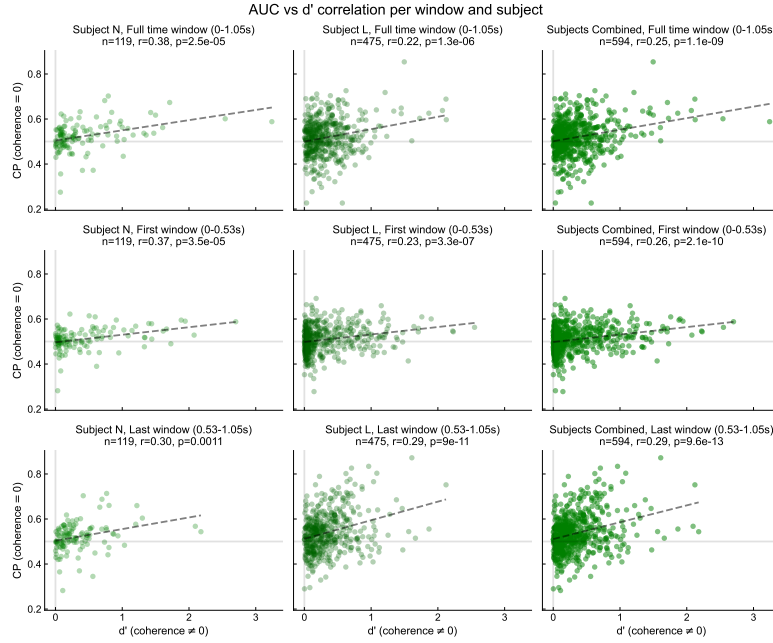
Fig. A5 Correlation between CP raw and d' .
