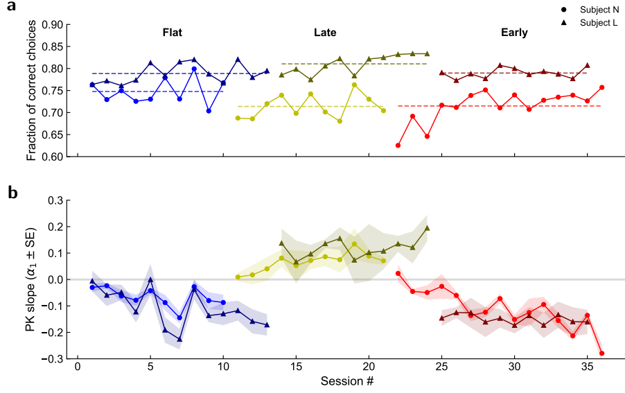
Fig. A1 Choice behavior of the two subjects. a. Average fraction of choices reporting correct motion direction across sessions. b. Slope of the psychophysical kernels ( \pm \text{SE} ) for the seven pulses [14] shown in Fig. 1c, computed by regressing \mathbf{y} = [\beta_1, \beta_2, \dots, \beta_7] via \mathbf{y} = \alpha_0 + \alpha_1 \mathbf{x} , \mathbf{x} = [1, 2, 3, 4, 5, 6, 7] .
