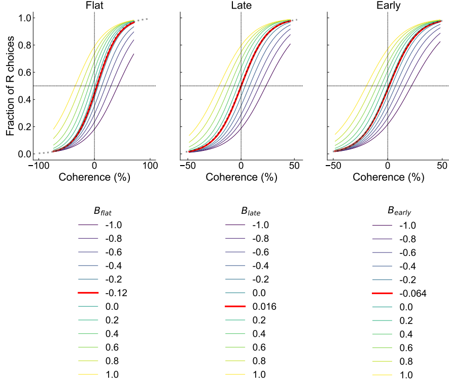
Fig. A14 Effects of varying B_{flat} , B_{late} , B_{early} on choice estimation. The parameters and \sigma_{flat} = 0.498 , \sigma_{late} = 0.531 , \sigma_{early} = 0.583 were kept fixed in the respective condition. Red indicates model output for optimized parameters; dotted lines indicate logistic fits on behavioral data.
