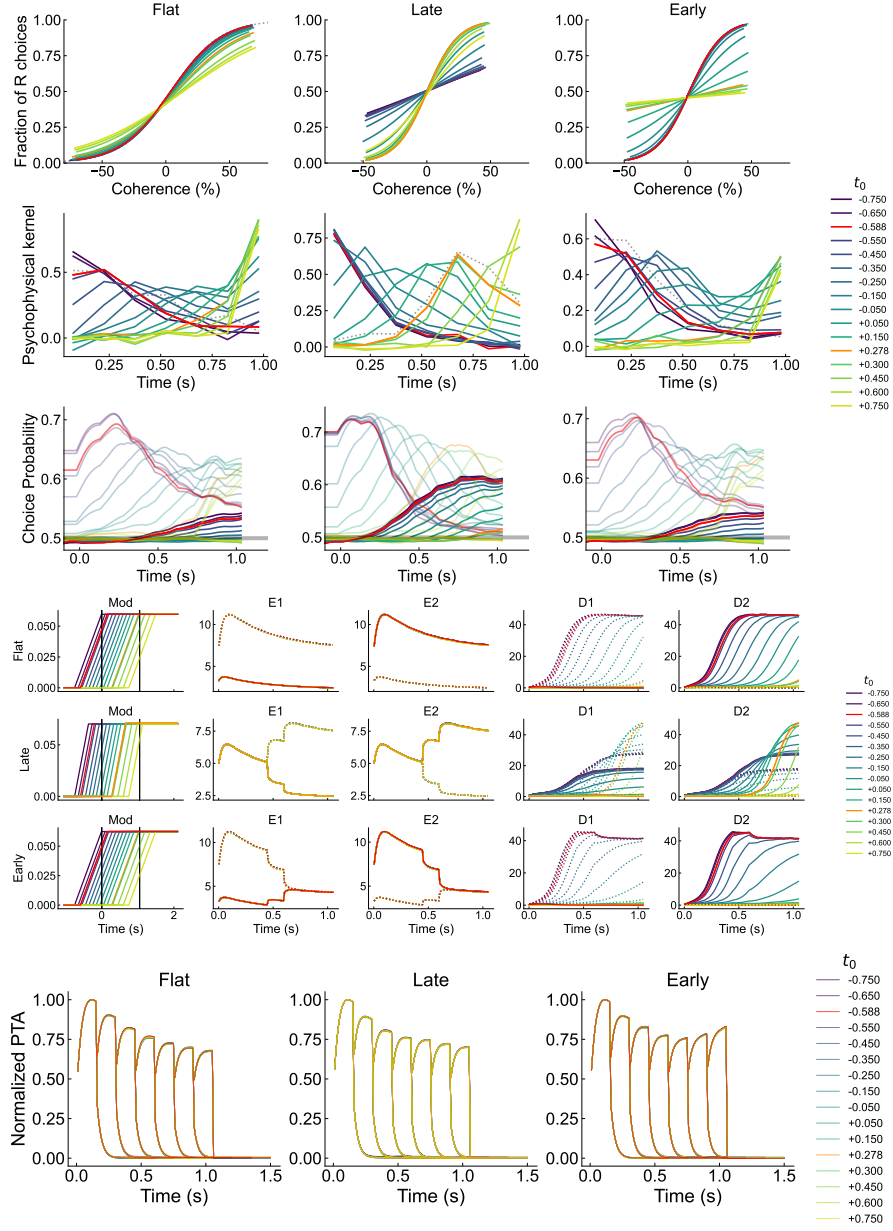
Fig. A12 Effects of varying t_{0,e} + t_{\text{offset}} , t_{\text{offset}} \in [-1.05, +1.15] (s) in e = \{\text{flat}, \text{late}, \text{early}\} . Red indicates model output for optimized parameter in flat and early conditions; orange indicates model output for optimized parameter in late condition. In CP plots, dotted lines indicate raw CP, solid lines indicate corrected CP. In firing rate plots, dotted lines indicate tuning to target 1, solid lines indicate tuning to target 2.
