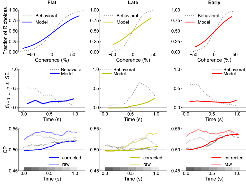
Fig. A9 Equivalent results for weaker feed-forward connectivity. Same as Fig. 3 but tuning connectivity weights to get raw CP (shaded colors in bottom row) within ranges comparable with MT data (gray in bottom row). We set J_{FF,1} = J_{FF,2} = 0.15 to show that it drastically impacts choice estimation (top row) and the magnitude of PKs (middle row). We also set the J_{FB,1} = J_{FB,2} = 0.001 to match such changes and recover the qualitative shape of raw and corrected CPs.
