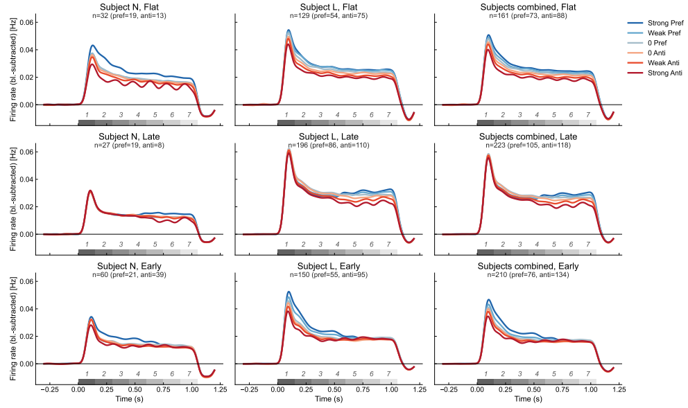
Fig. A2 Showing results in 2a for the two subjects separately.
