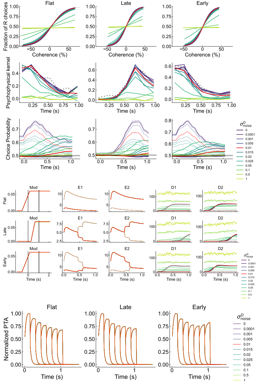
Fig. A20 Effects of varying \sigma_{\text{noise}}^D . Red indicates model output for optimized parameters. In CP plots, dotted lines indicate raw CP, solid lines indicate corrected CP. In firing rate plots, dotted lines indicate tuning to target 1, solid lines indicate tuning to target 2.
