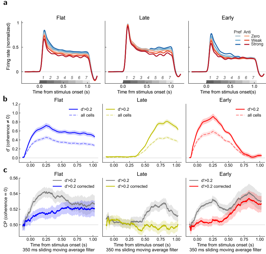
Fig. 2 Stimulus and choice selectivity in MT. a. Baseline-subtracted, peak-normalized firing rates for the respective cumulative motion strengths (darker for strong, lighter for weak and zero coherence) and choice preference tuning (preferred in blue, or anti-preferred in red) in the three stimulus conditions. Population firing rates were baseline-subtracted by subtracting the mean pre-stimulus firing rate from each cell's firing rate and normalized to their peak response across trials. Traces show the mean across cells and trials and were smoothed using a Gaussian kernel ( \sigma = 25 ms). Averages are reported across all cells ( n = 161 Flat, 223 Late, 210 Early), aligning neurons according to their preferred direction (preferred right: n = 80 flat, n = 108 late, n = 82 early; preferred left: n = 81 flat, n = 115 late, n = 128 early). Separate results for the two subjects are shown in Supp. Fig. A2. b. Time-resolved motion discriminability ( d' mean \pm SEM across sessions) for preferred motion direction vs. the opposite direction in the three stimulus conditions. Results are shown for all cells ( n = 161 Flat, 223 Late, 210 Early) and for cells showing epoch-wise d' > 0.2 ( n = 84 Flat, 87 Late, 116 Early), computed on the time-averaged firing rate during stimulus presentation time (Supp. Table A5). Results for the two subjects are shown separately in Supp. Fig. A3. c. Choice Probability (CP mean \pm SEM across sessions) for zero pulse-averaged coherence trials across sessions for each of the three temporal weighting conditions. CPs were computed from raw firing rates (gray) and by applying CP correction removing the effect of non-zero motion strength of single pulses on firing rates (colored). Results for all cells and for each subject are shown in Supp. Fig. A4. b–c. All time-resolved analyses are computed using a moving spike rate window of width T = 350 ms sliding with step 1 ms.
