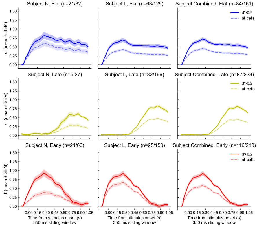
Fig. A3 Subject-specific d' . Showing results in 2b for the two subjects separately. In parentheses, we indicate the number of cells showing epoch-wise d' > 0.2 out of the total number of cells available.
