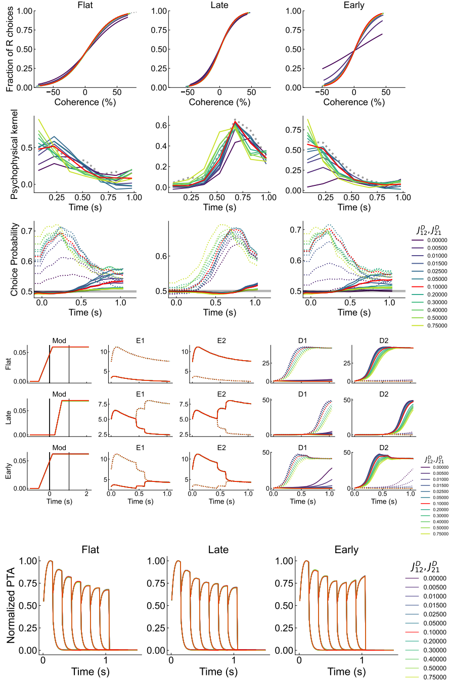
Fig. A18 Effects of varying J_{12}^D = J_{21}^D . Red indicates model output for optimized parameters. In CP plots, dotted lines indicate raw CP, solid lines indicate corrected CP. In firing rate plots, dotted lines indicate tuning to target 1, solid lines indicate tuning to target 2.
