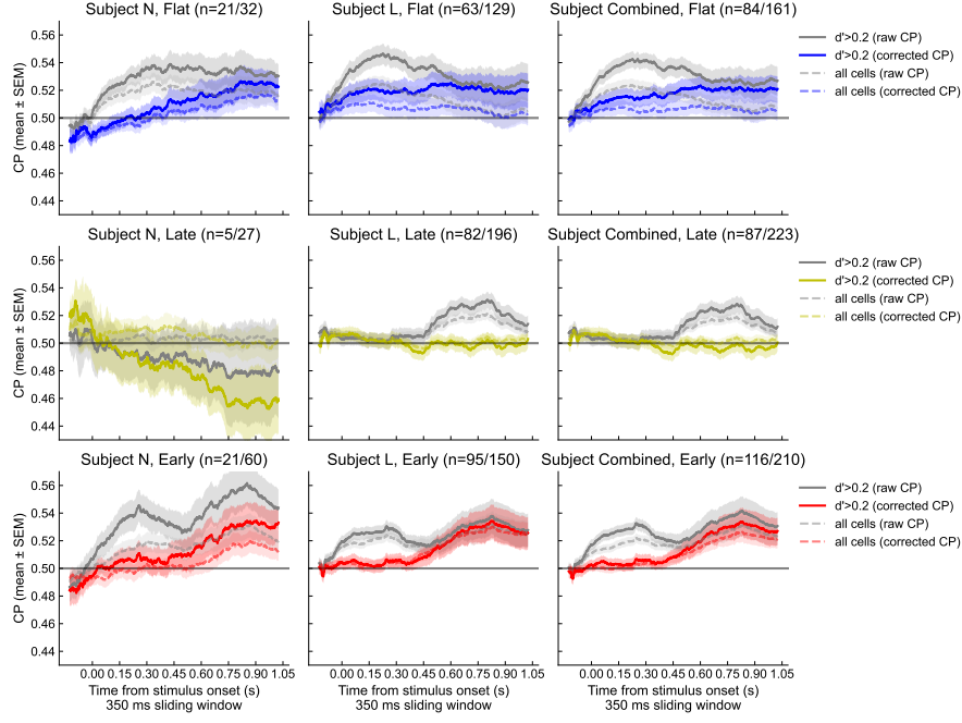
Fig. A4 Subject-specific CP. Showing results in 2c for all available cells and for the two subjects separately. In parentheses, cells showing epoch-wise d' > 0.2 out of the total number of cells available.
