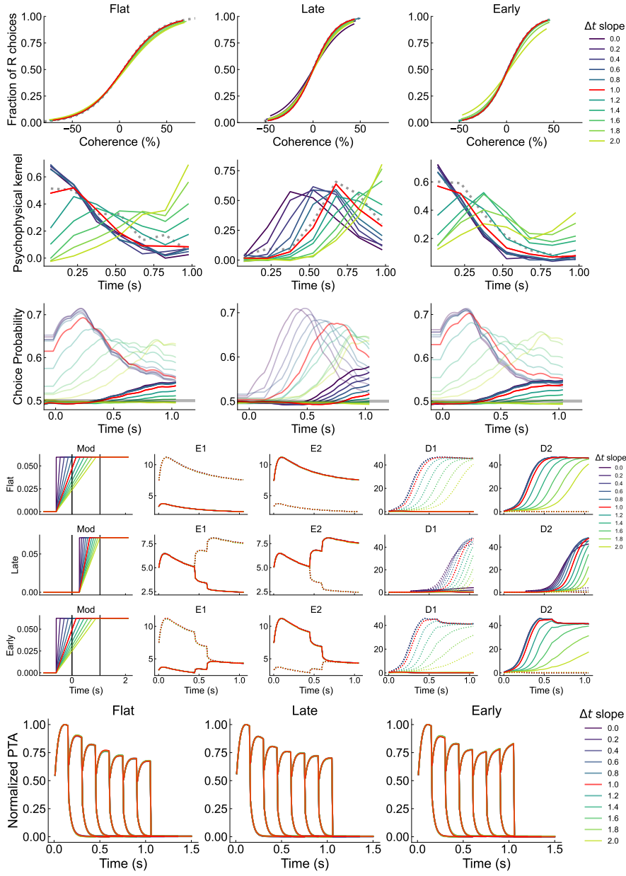
Fig. A13 Effects of varying I_{\text{mod}} slope as k\Delta t_e , k \in [0, 2] (s) for e = \{\text{flat, late, early}\} . Red indicates model output for optimized \Delta t_e ( k = 1 ). In CP plots, dotted lines indicate raw CP, solid lines indicate corrected CP. In firing rate plots, dotted lines indicate tuning to target 1, solid lines indicate tuning to target 2.
