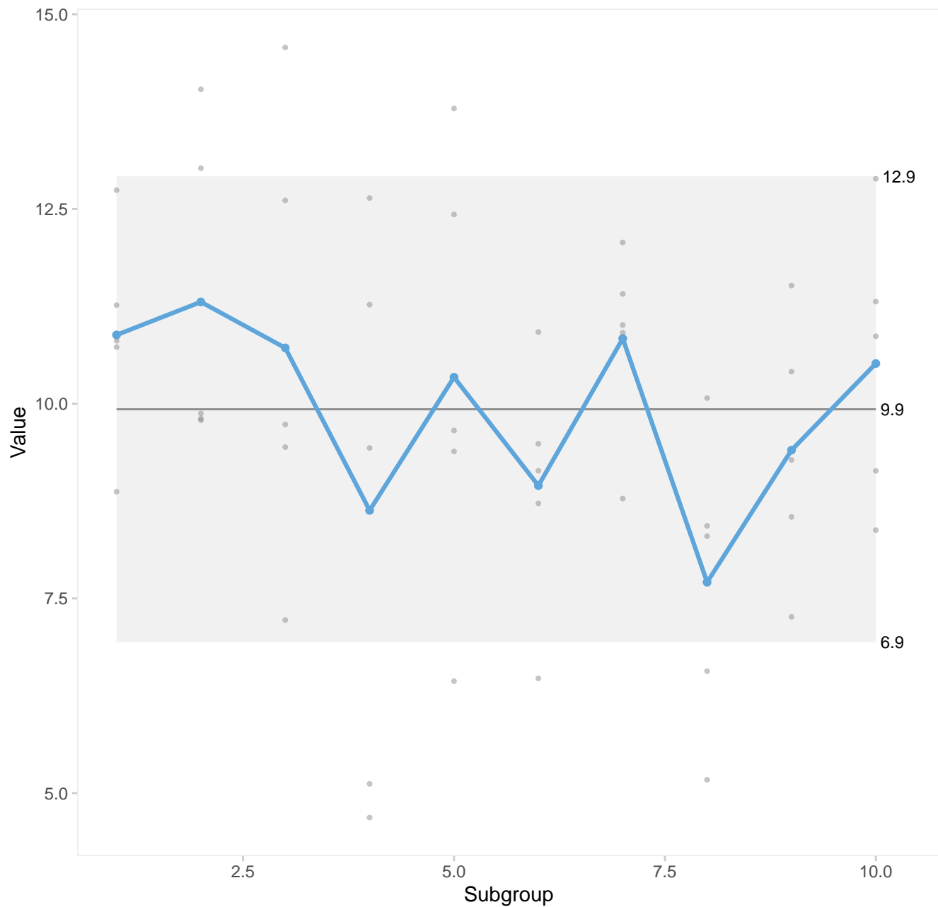
Xbar Chart (with raw data)
