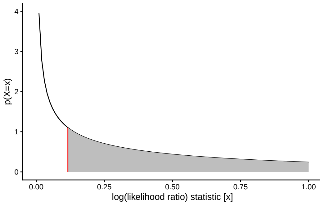
Figure 9: Chi-square distribution
