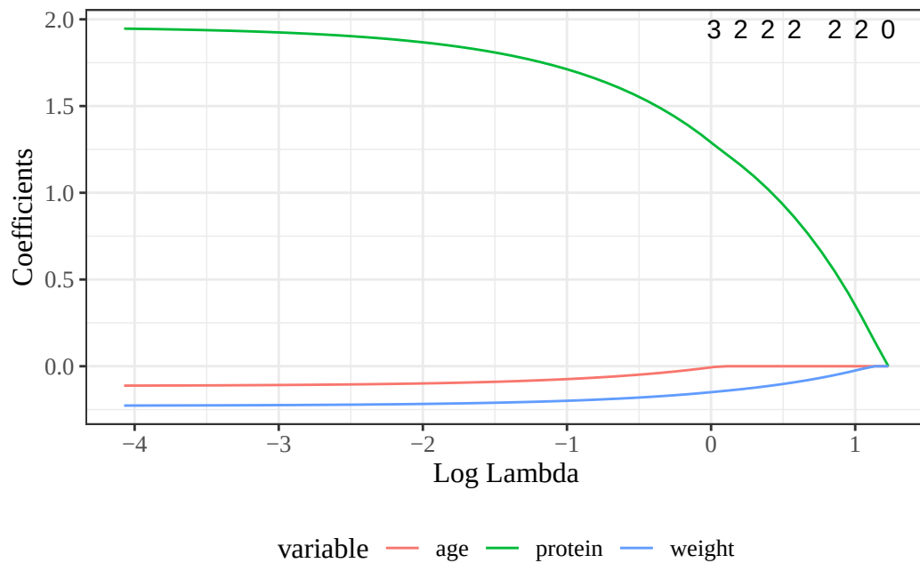
Figure 34: Lasso selection
