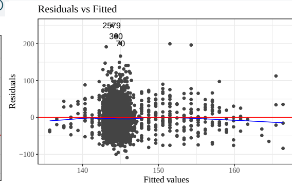
(b) with intercept term
