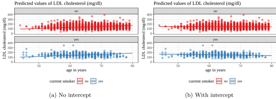
Figure 14: hers data models with and without intercepts
