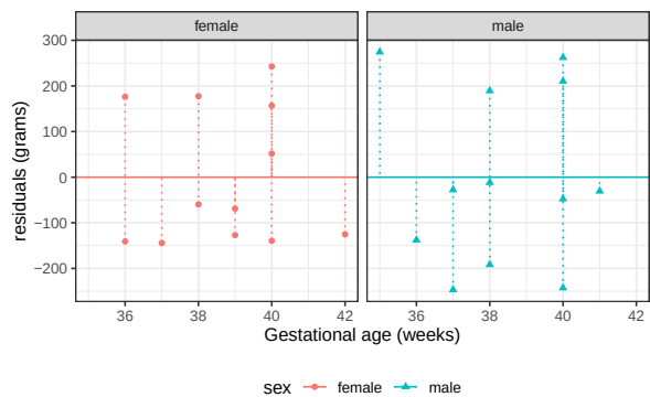
(b) Residuals
