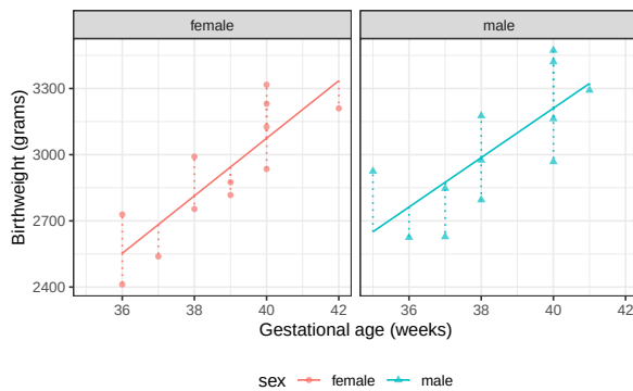
(a) fitted values
