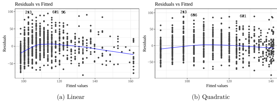
Figure 25: Residuals versus fitted plot for linear and quadratic fits to PLOS data
