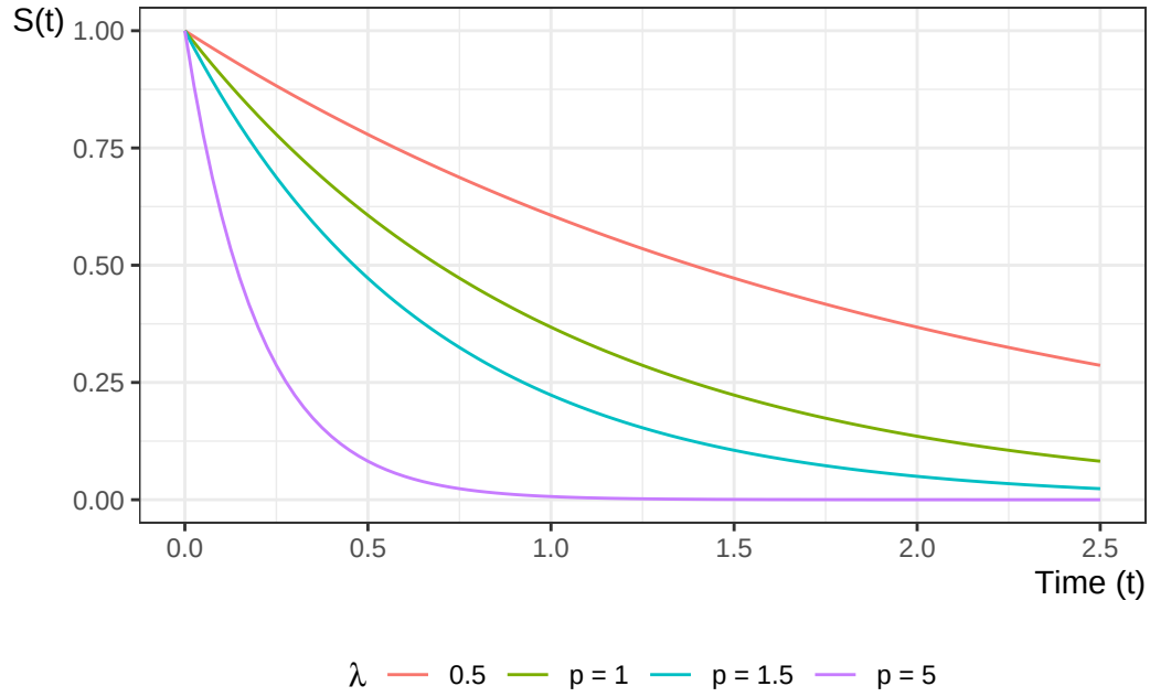
Figure 1: Exponential Survival Functions
