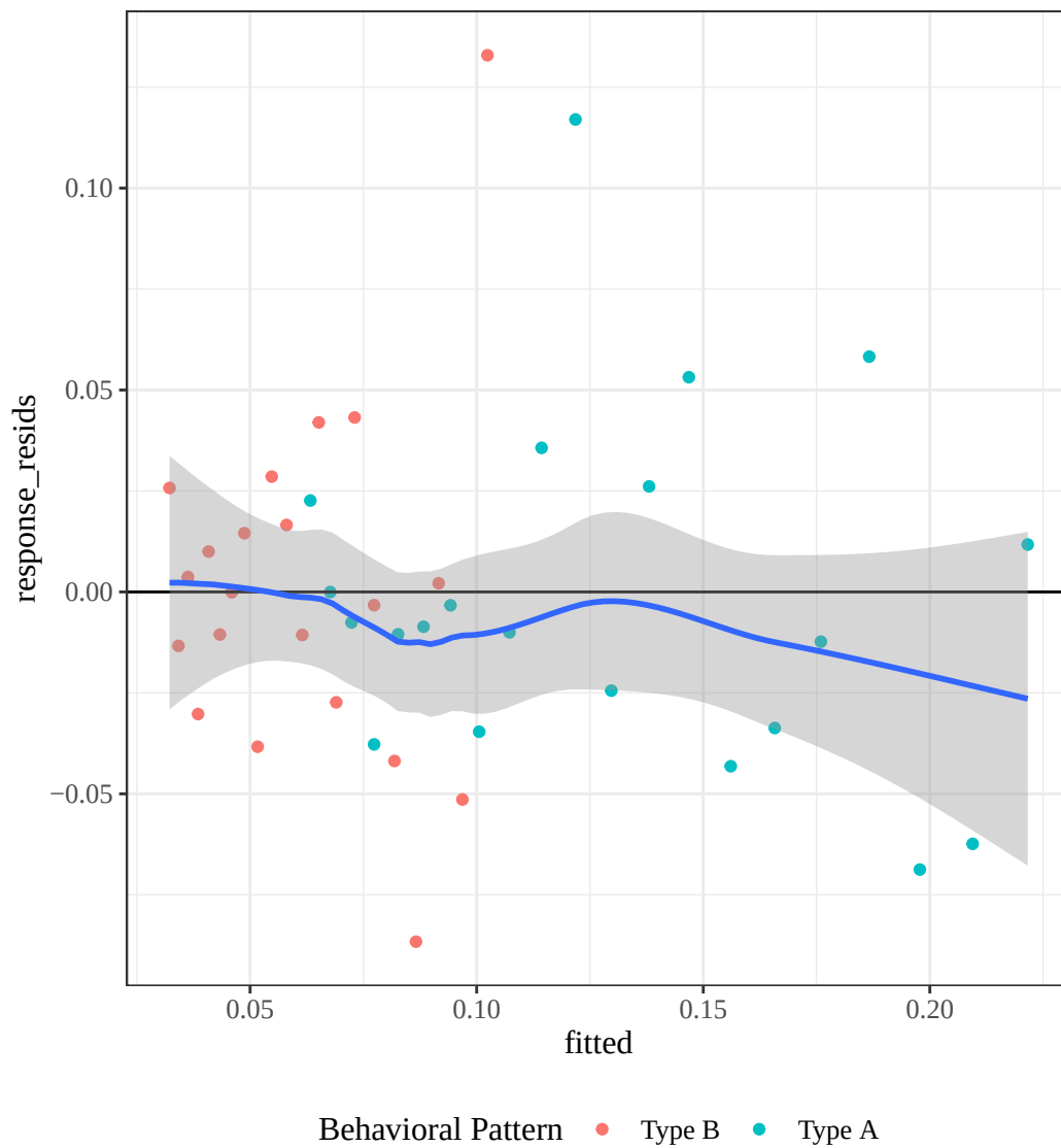
Figure 18: residuals plot for wgs model
