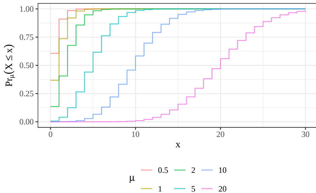
Figure 3: Poisson CDFs
