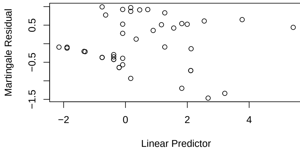
Figure 15: Martingale Residuals vs. Linear Predictor
