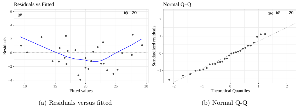
Figure 51: Diagnostic plots for linear model fit to mtcars data
