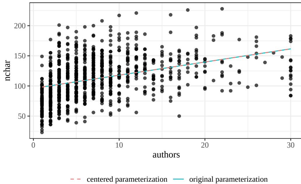
Figure 50: PLOS data with original and centered parameterizations
