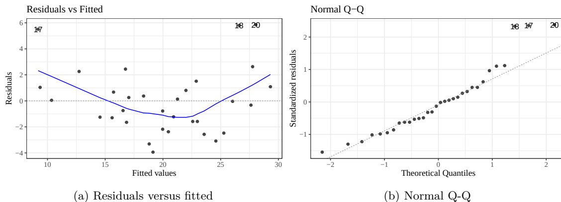
Figure 51: Diagnostic plots for linear model fit to mtcars data
