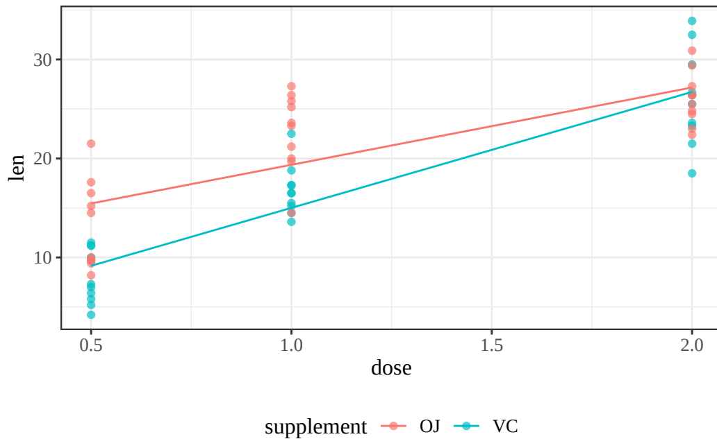
Figure 49: ToothGrowth data with interaction (non-parallel-lines) fit
