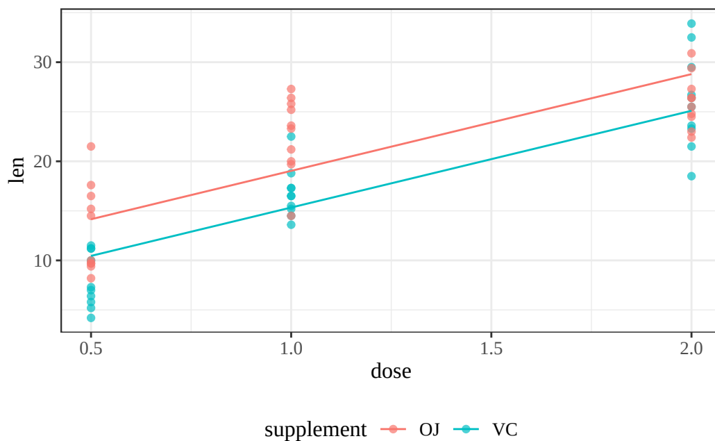
Figure 48: ToothGrowth data with additive (parallel-lines) fit
