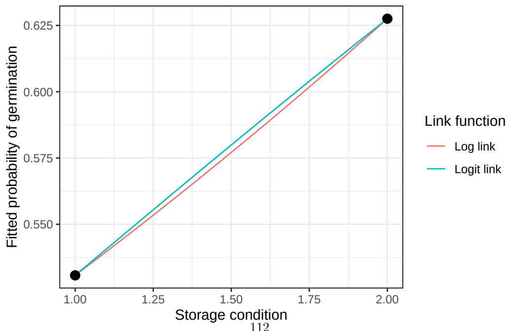
Figure 18: Fitted germination probabilities from the log-link and logit-link models for the anthers data, with the observed proportions as points. The two link functions nearly coincide here because
