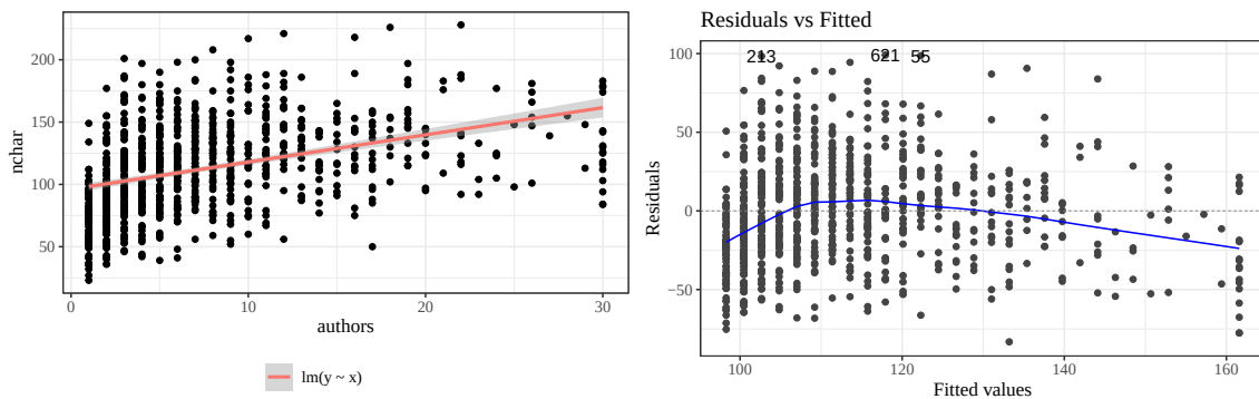
Figure 23: Number of authors versus title length in PLOS Medicine , with linear model fit
