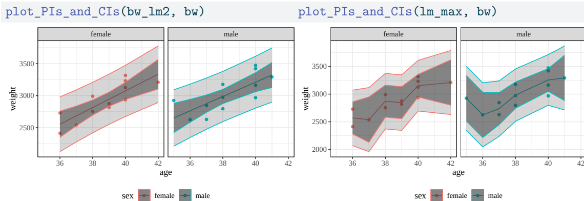
Figure 7: Model 2 and saturated model for birthweight data, with confidence and prediction intervals
