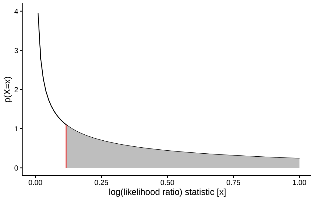
Figure 8: Chi-square distribution
