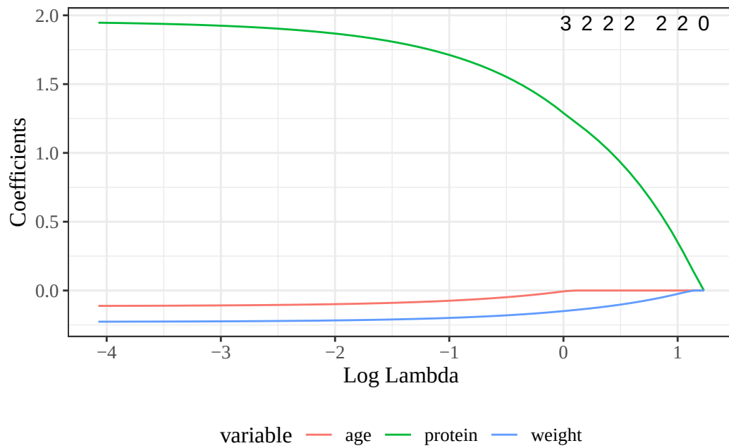
Figure 36: Lasso selection
