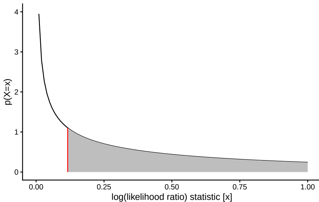
Figure 11: Chi-square distribution
