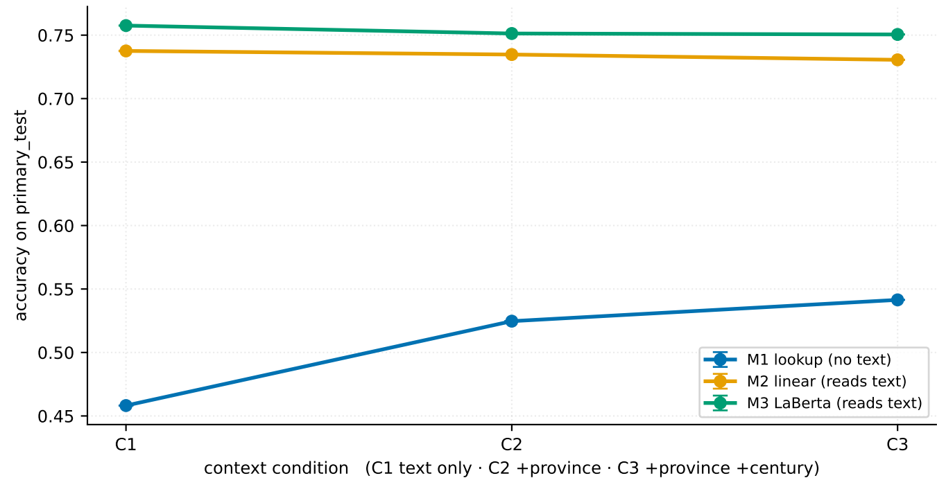
Province and century help only a model that cannot read the text
