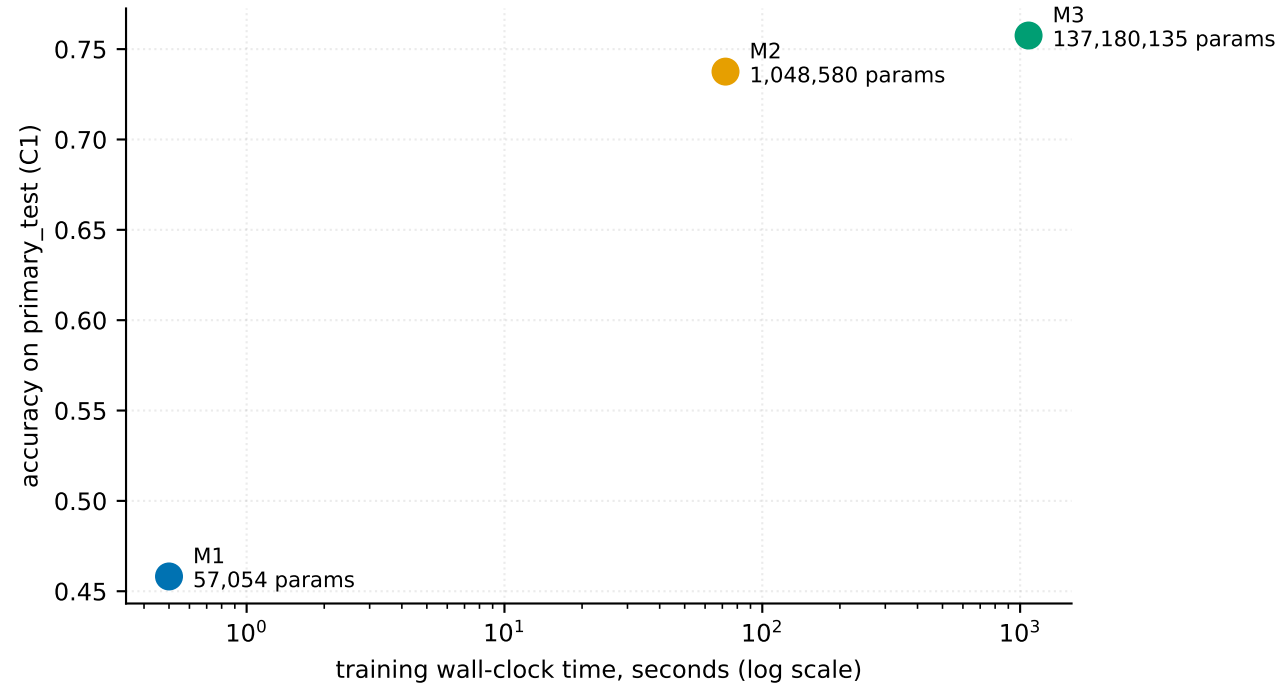
A linear model recovers 97% of a Latin transformer's accuracy
