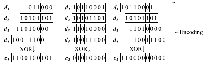
图 2-1 Two-tone 码编码举例 ( k = 4, m = 3 )
