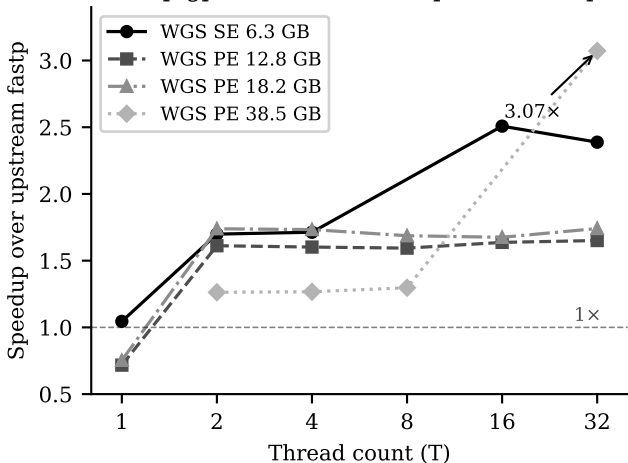
fastp-gpu CPU mode vs. upstream fastp
