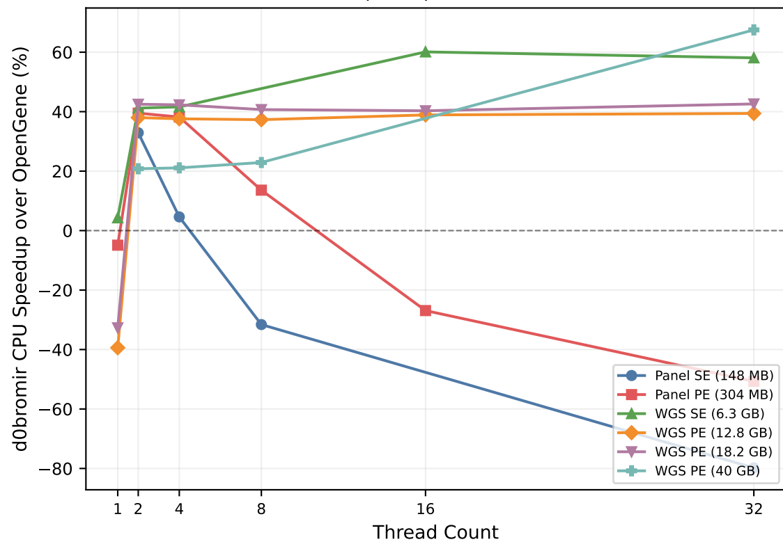
(b) CPU Speedup vs Thread Count
