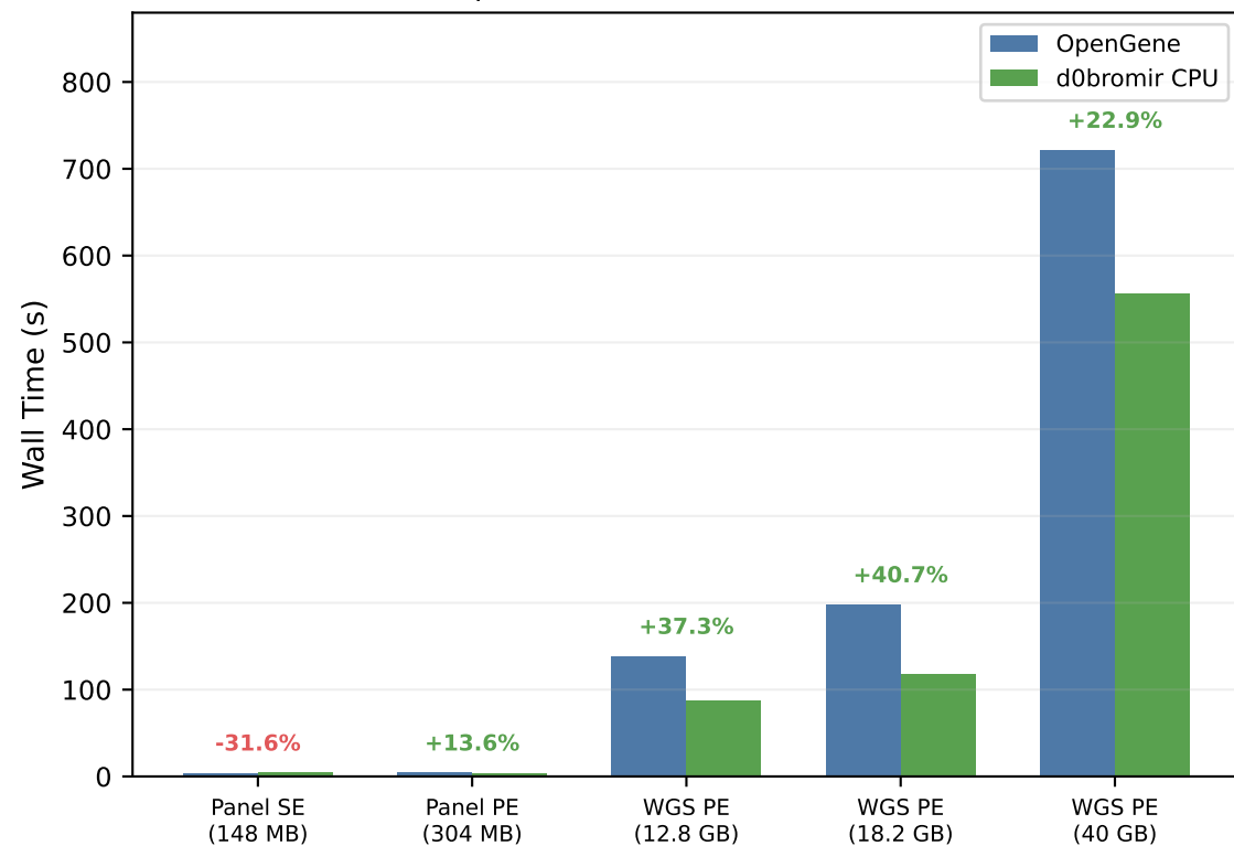
(a) OpenGene vs d0bromir CPU at T=8
