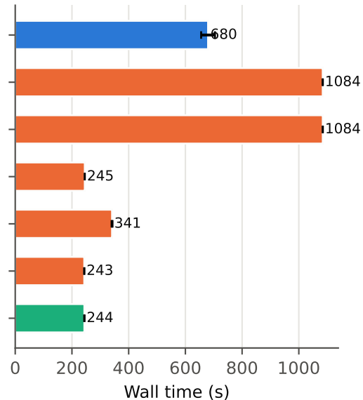
32 threads
