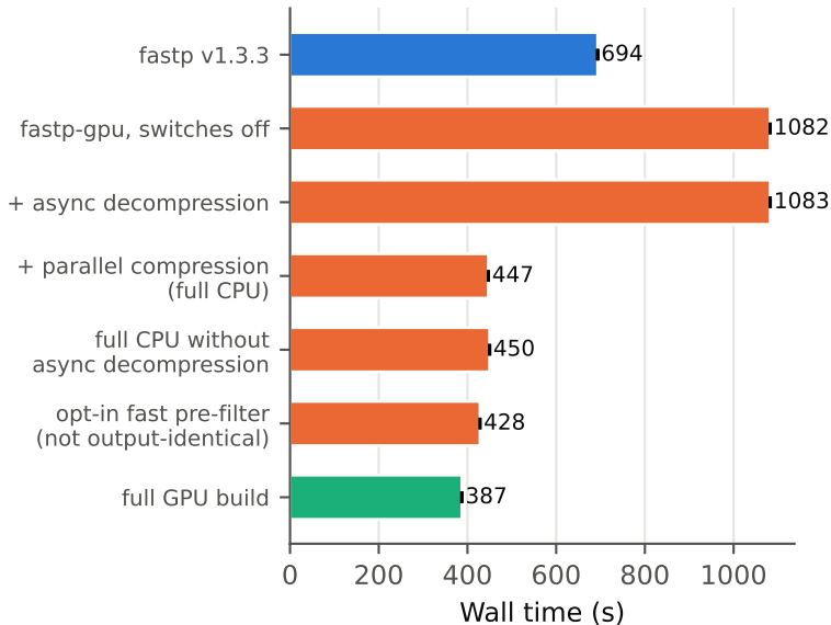
8 threads
