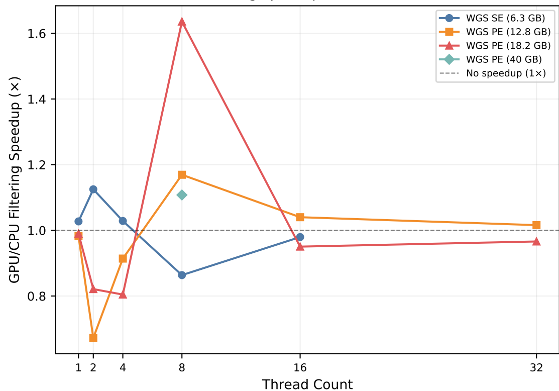
(b) Filtering Speedup vs Thread Count
