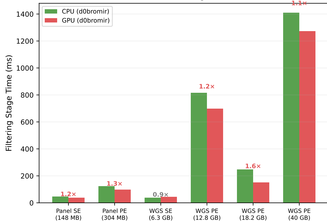
(a) CPU vs GPU Filtering Time at T=8
