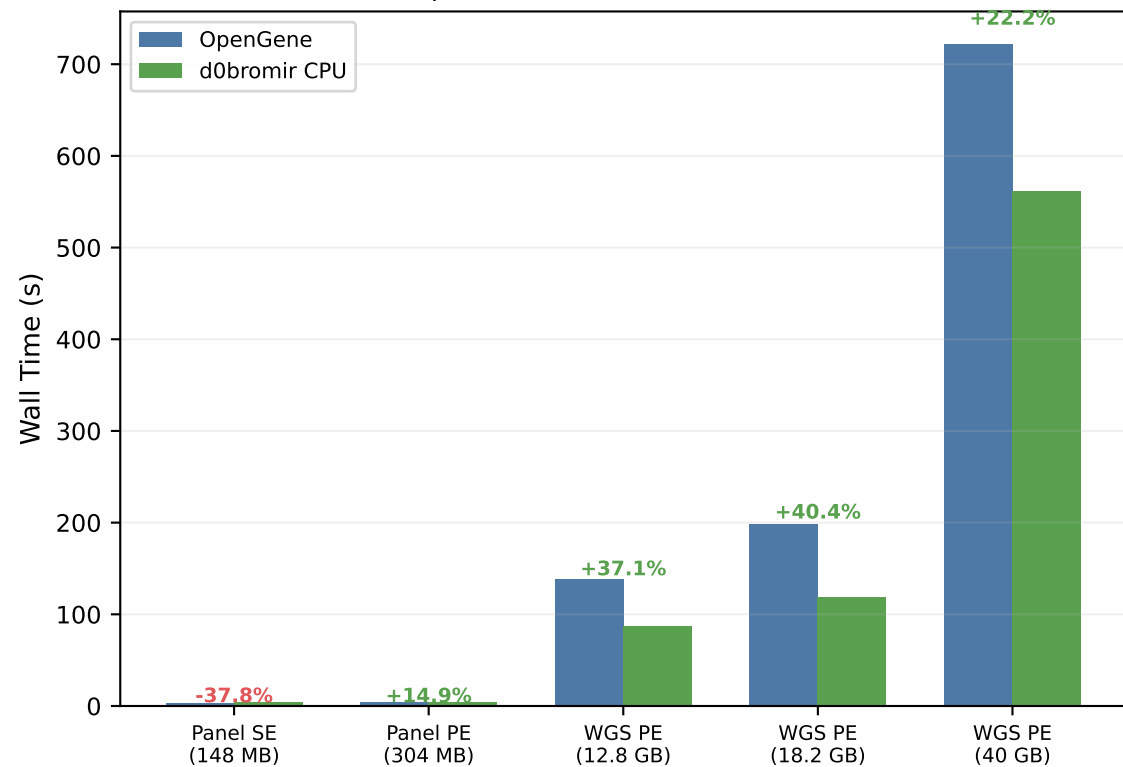
(a) OpenGene vs d0bromir CPU at T=8
