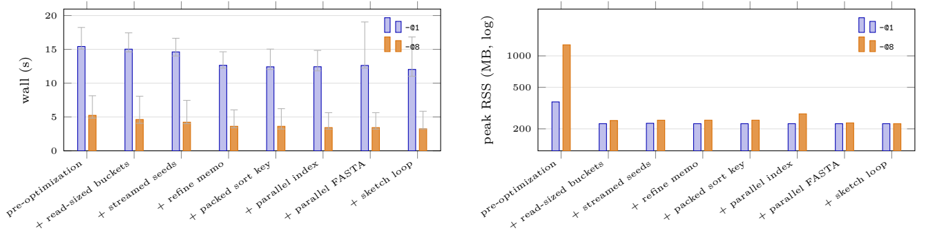
Figure 1: Every optimization, put back one at a time. Rung pre-optimization runs the shipped binary with every ablatability change switched off ( SHMAP_ABLATE , src/ablate.rs ); each rung to its right switches exactly one more back on, in the layer order this note argues. Adjacent rungs therefore differ by one change and nothing else — same binary, machine, compiler and input — so a step is that change’s worth given the ones before it , which is the only sense in which these interacting changes have individual values. The two series are the two thread counts; the gap between them is row 4, threaded read mapping, which is a capability rather than a branch and so cannot be a rung. Row 8 is type- and build-level and is not ablated at all. Left: wall clock, bars at the median over 9 runs of the whole ladder and whiskers at min–max, so a step this host has not resolved is visible as one. The two parallelism rungs cannot move the one-worker series at all — at -01 both take the serial path in either position — so their flat steps there are structure, not noise. Right: peak resident set — one worker’s genome-sized accumulator hides under the index-build peak, but -08 workers’ copies do not, which is the scaling argument in one picture. Every rung’s mapping is byte-identical; the run fails otherwise. Numbers, per-stage timers and the spread behind every bar in figure_ablation.tsv .
