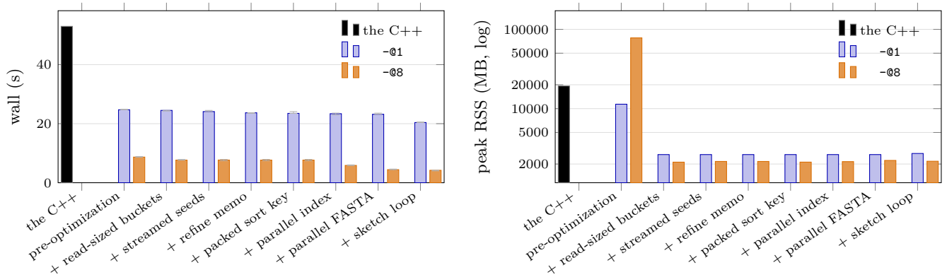
Figure 2: Every optimization, put back one at a time, on the whole genome (D6-ONT24K, REF-HS1). The leftmost bar is the C++ itself; pre-optimization is this port with every ablatability change switched off (SHMAP_ABLATE), and each rung to the right switches exactly one more back on, so adjacent rungs differ by one change and nothing else. End to end the C++ is 2.64× the shipped mapper here, of which 2.15× is the port itself and 1.23× the ladder; the product returns the first. The two series are the two thread counts: their gap is row 4, row 8 is not ablatable, and the C++ has no -0N counterpart. Left: wall clock, median of 5 round-robin runs of the whole ladder, whiskers at min-max. Right: peak resident set, log scale; the accumulator the first change removes is sized by the reference and allocated per worker , which is why the -08 baseline stands above even the C++. Every rung’s mapping is byte-identical; the run fails otherwise. Numbers, per-stage timers and the decomposition in figure_ablation.tsv and reconcile.tsv .
