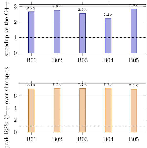
Figure 1: The two headline results, per benchmark, single-threaded on both sides: wall-clock speedup over the C++ (top) and how many times less peak memory the port uses (bottom). The dashed line is parity.
