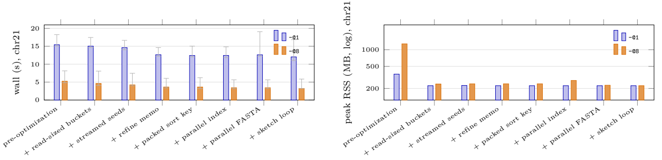
Figure 2: Every optimization, put back one at a time, on a 45 Mbp chromosome — so these are relative worths, not the whole-genome result, which is Figure 1. pre-optimization is this port with every ablatable change switched off (SHMAP_ABLATE); each rung to the right switches exactly one more back on, so adjacent rungs differ by one change and nothing else. Getting from the C++ to pre-optimization is worth a further 1.67 \times , measured against both in one sitting rather than drawn here, because the C++ takes no -x and these rungs do. The two series are the two thread counts, and the gap between them is row 4; row 8 is not ablatable. Left: wall clock, median over 9 round-robin runs of the whole ladder, whiskers at min-max, so an unresolved step is visible as one. Right: peak resident set, log scale — one worker’s genome-sized accumulator hides under the index-build peak, -@8 workers’ copies do not. Every rung’s mapping is byte-identical; the run fails otherwise. Numbers and per-stage timers in figure_ablation.tsv ; the decomposition against the C++ in reconcile.tsv .
